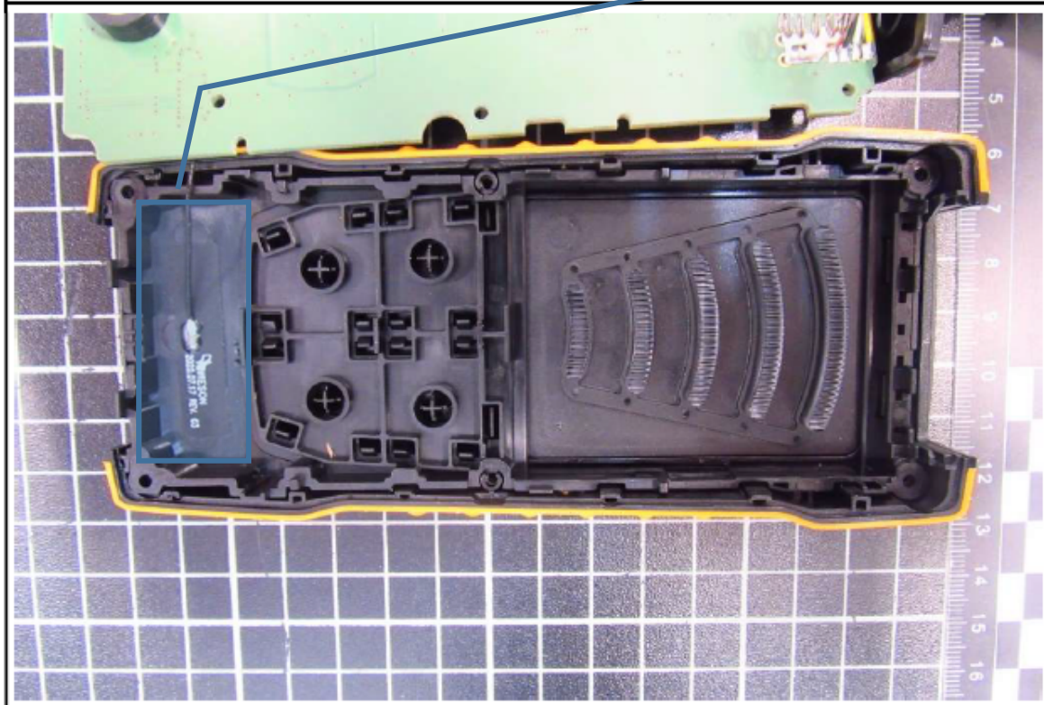
Interior view on front panel and BTLE antenna
