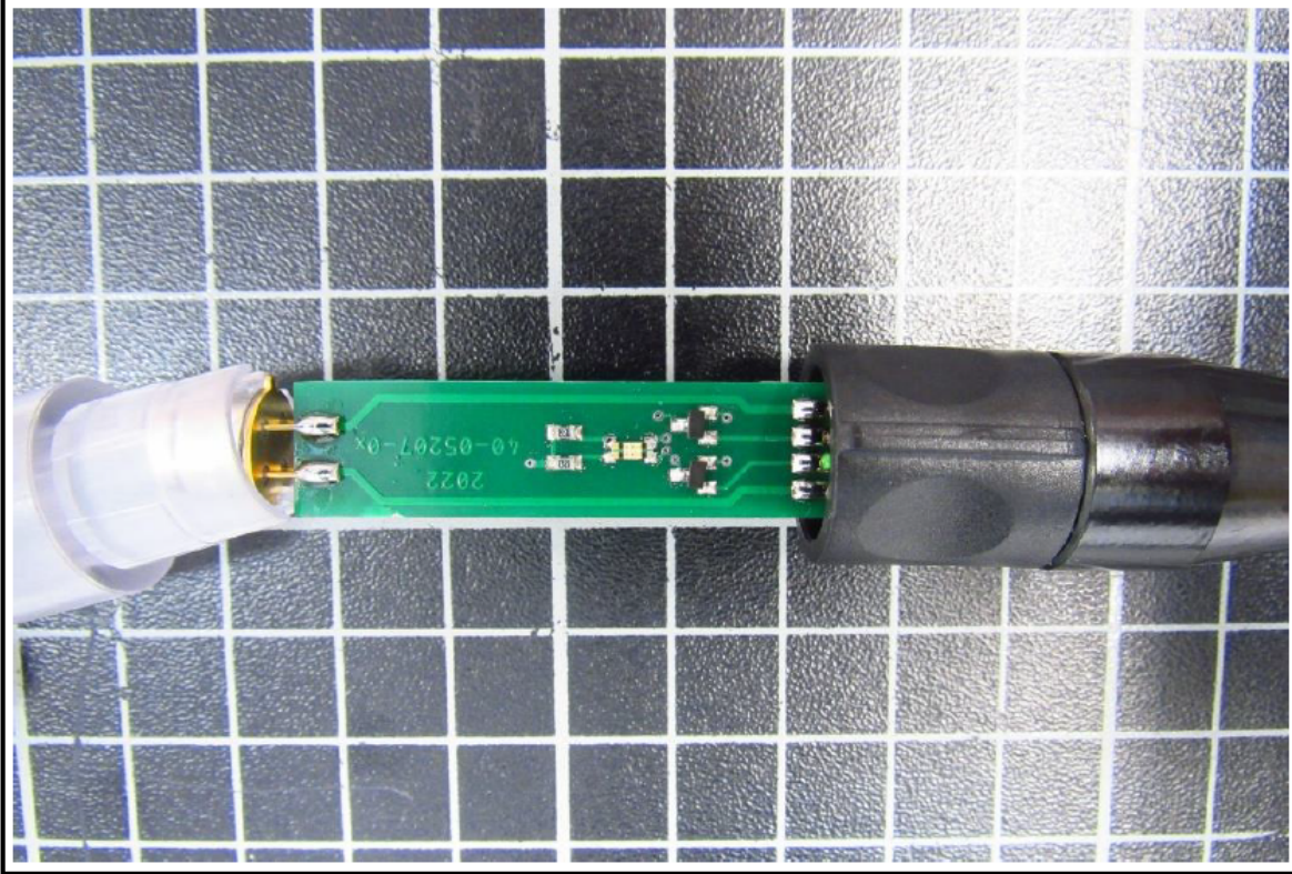
Sensor PCB bottom side view
