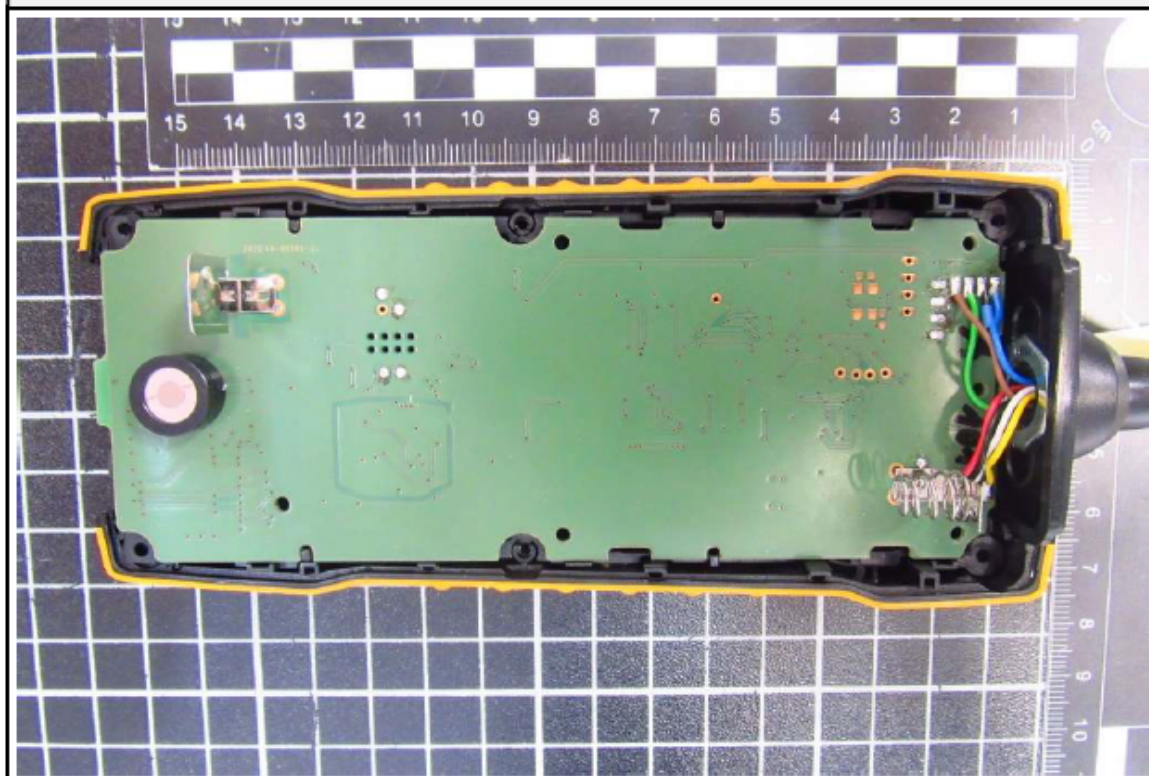
PCB top side view
