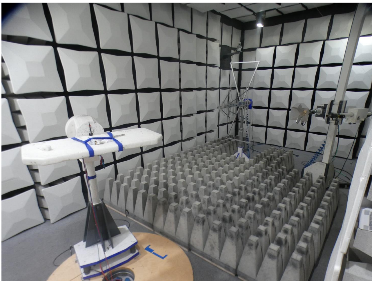
Photo 5: Test setup for radiated measurements (stand alone setup, 1 GHz – 24 GHz; FCC 15c247)
