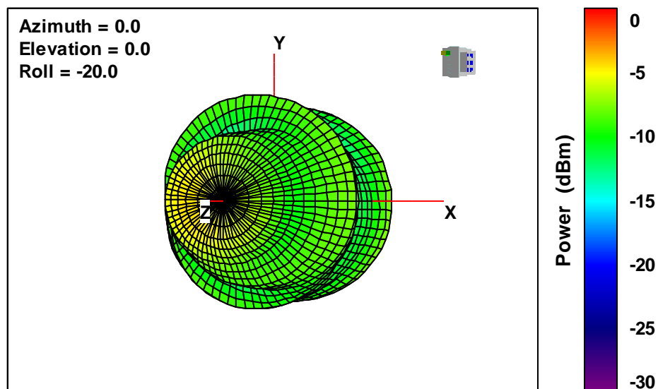
Fig. 5: 2480 MHz 3D Radiated pattern orientation of DUT compared to a phone.
