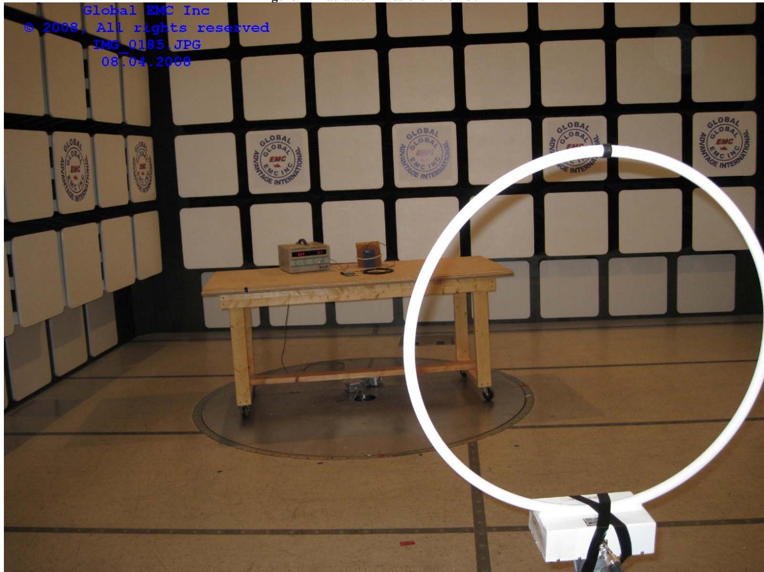
Figure 1 - Radiated Emissions Below 30 MHz
