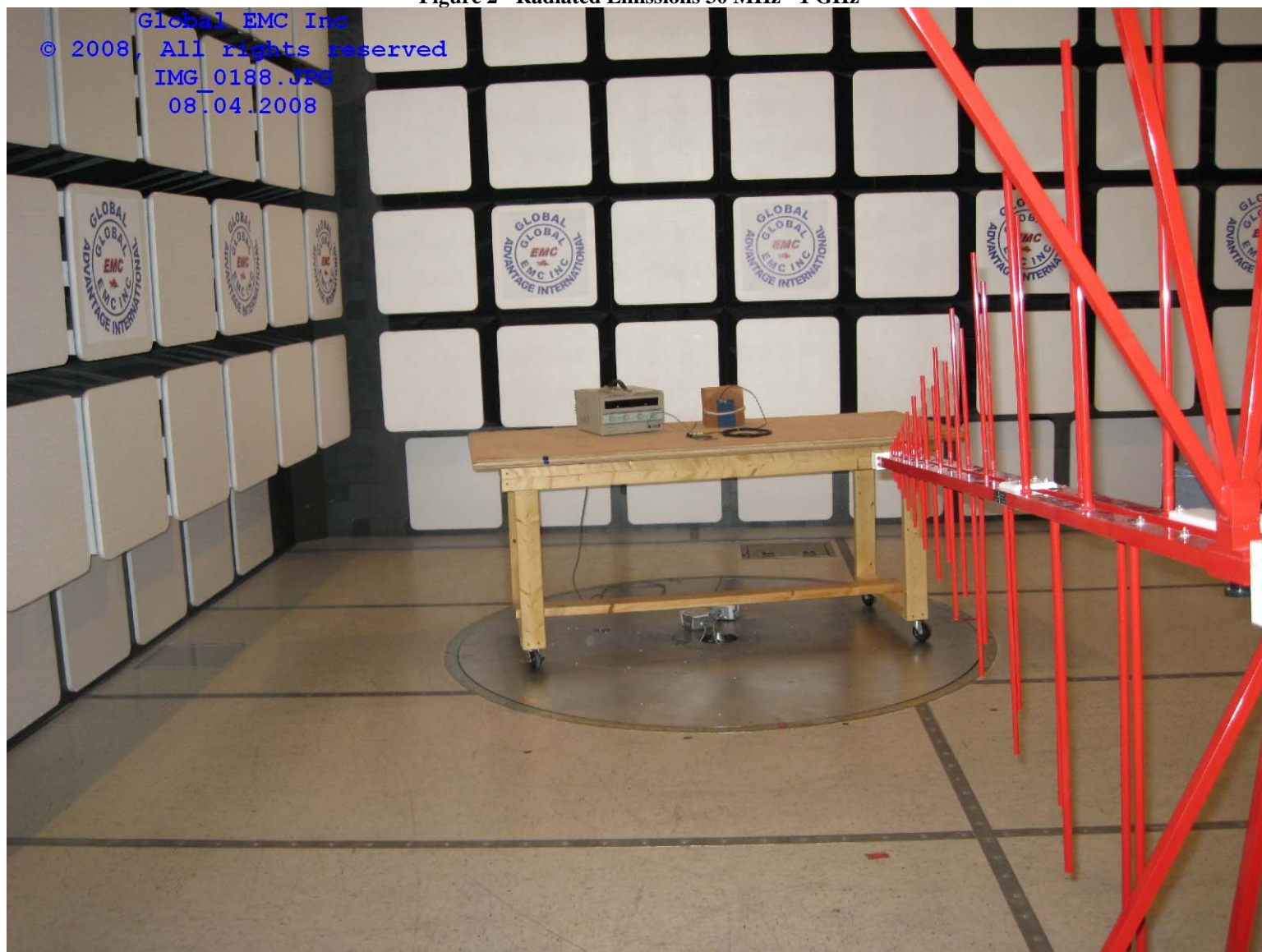
Figure 2 - Radiated Emissions 30 MHz - 1 GHz
