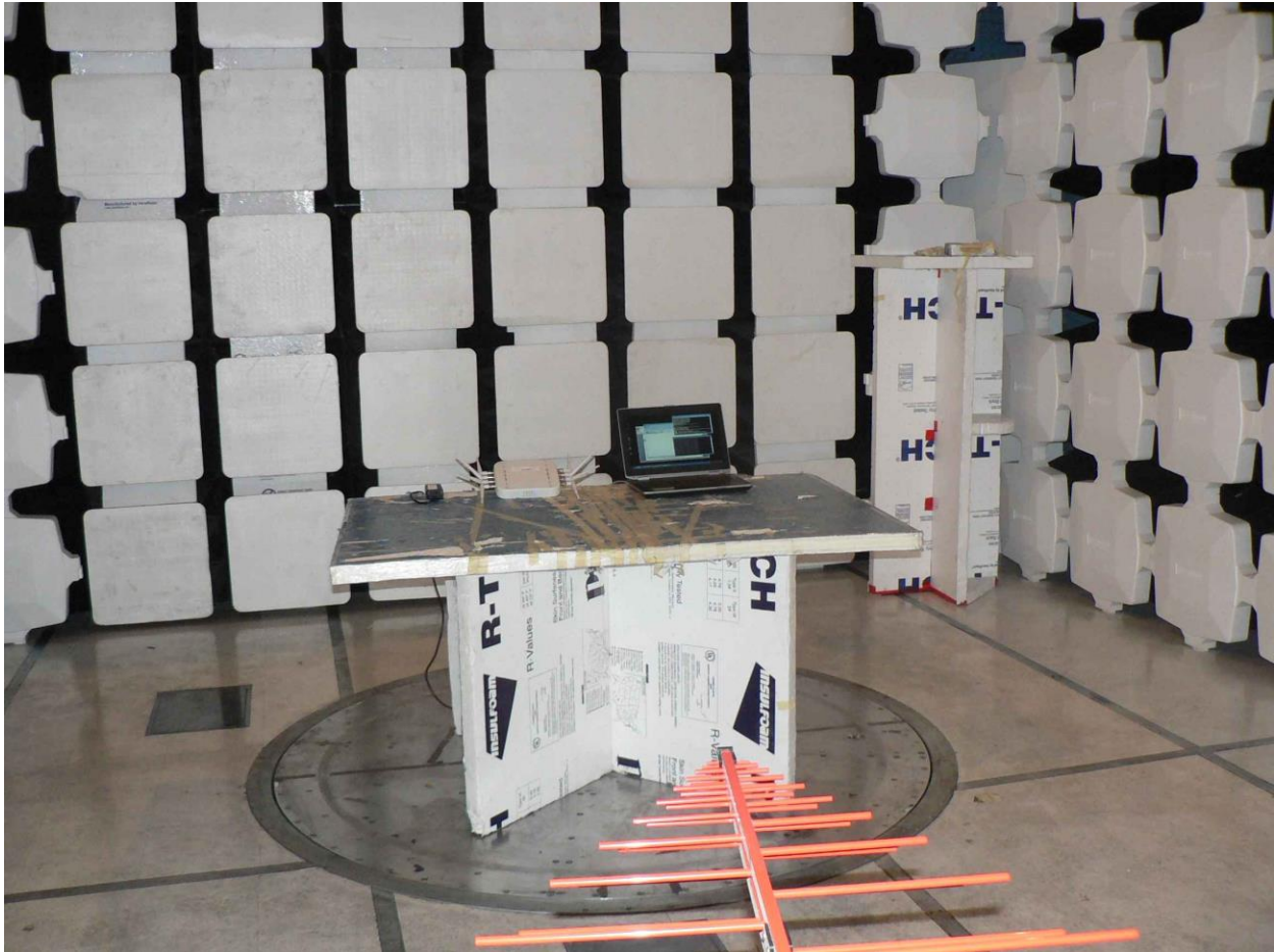
NTCT66 WiFi Ext Dig Em 30-1000 GC PS Front
