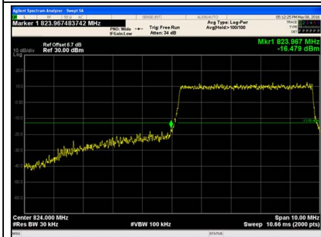
LTE Band 5 - Low Channel 16QAM-5
