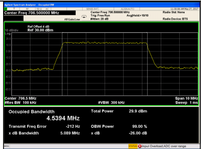
LTE Band XVII - Low CH 16QAM-5
