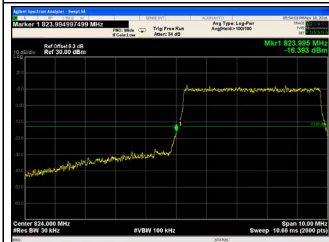
LTE Band V - Low Channel QPSK-5
