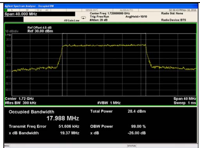
LTE Band IV - Low CH 16QAM-20
