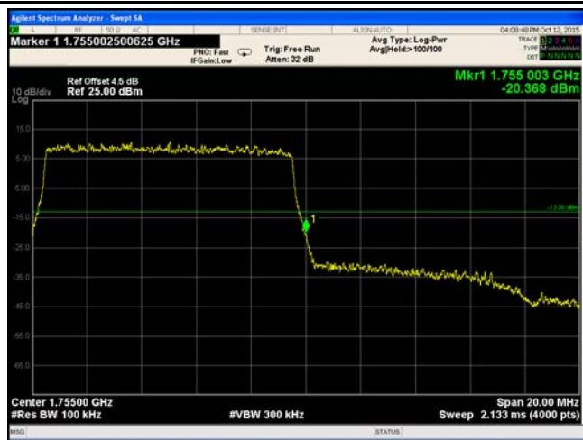
LTE Band 4 - High Channel 16QAM-10
