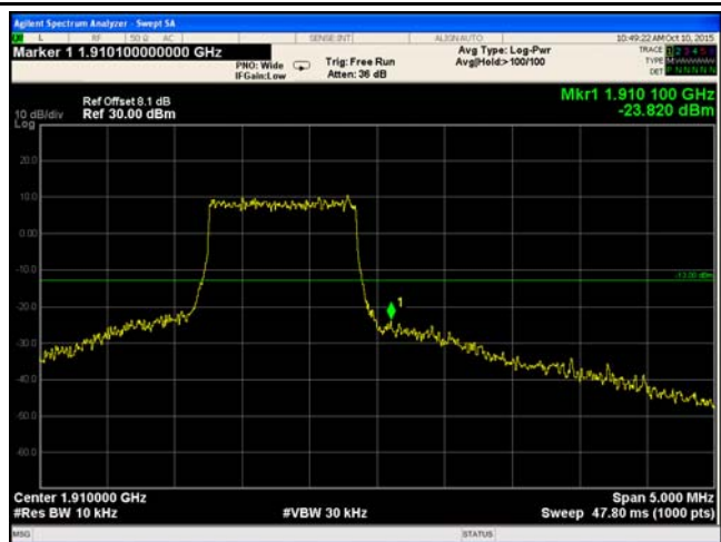
LTE Band 2 - High Channel 16QAM-1.4
