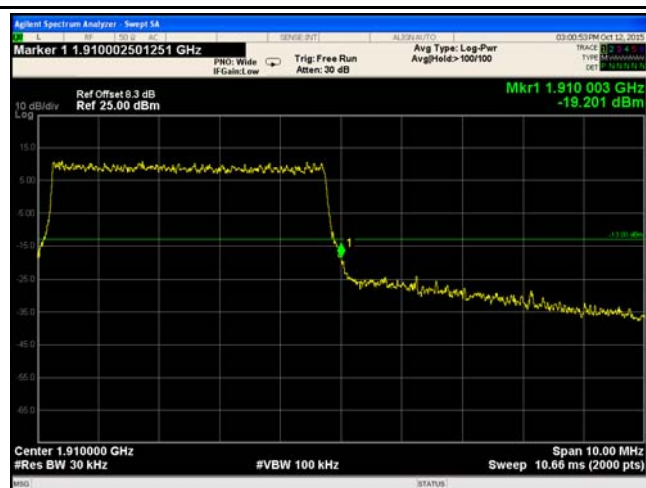
LTE Band 2 - High Channel QPSK-5
