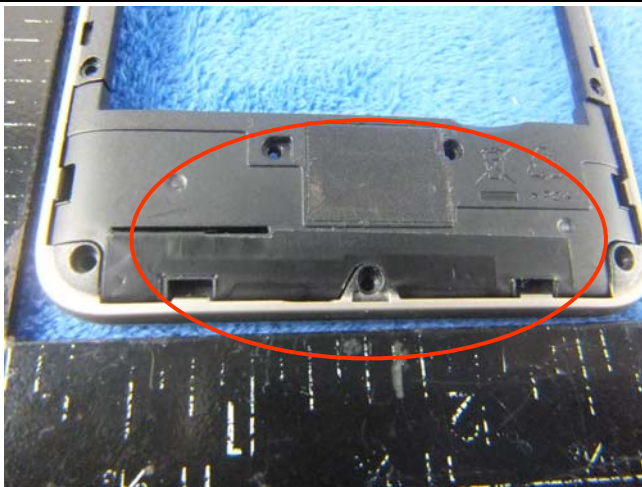
UMTS-FDD/GSM Antenna View
