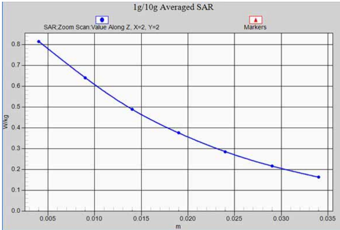
WCDMA Band V(Body)/Back side-Mid_ z-axis scan
