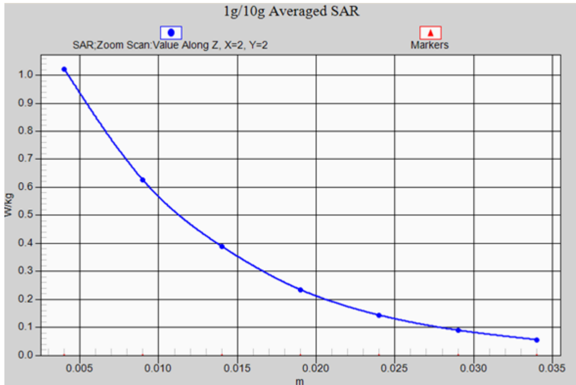
GPRS 1900/Back side-Low_ z-axis scan
