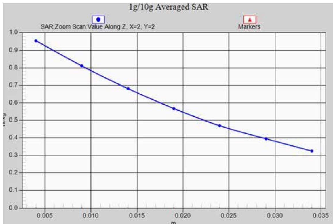
WCDMA Band II(Body)/Back side-Low_ z-axis scan
