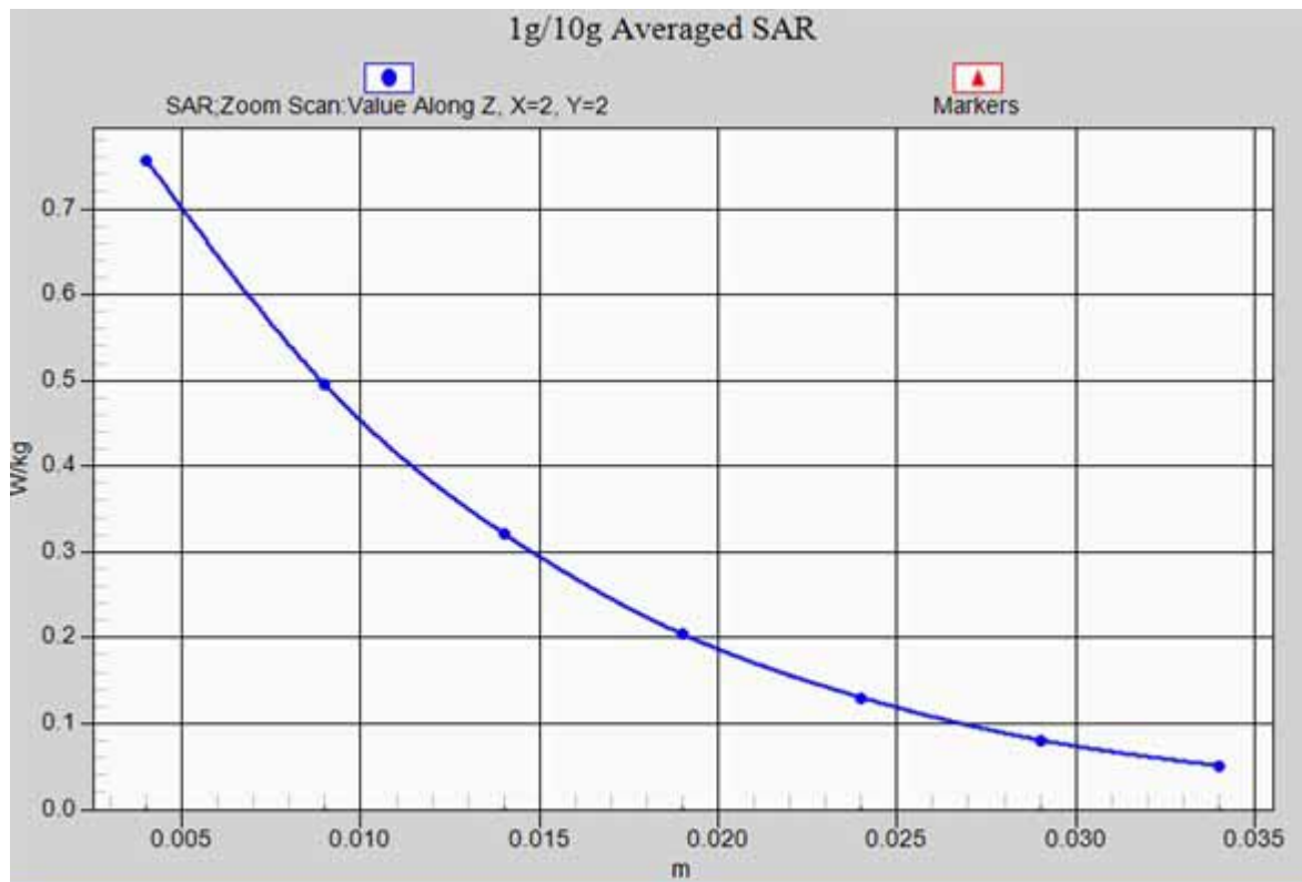
WCDMA Band II- LEFT/CHEEK-LOW_ z-axis scan
