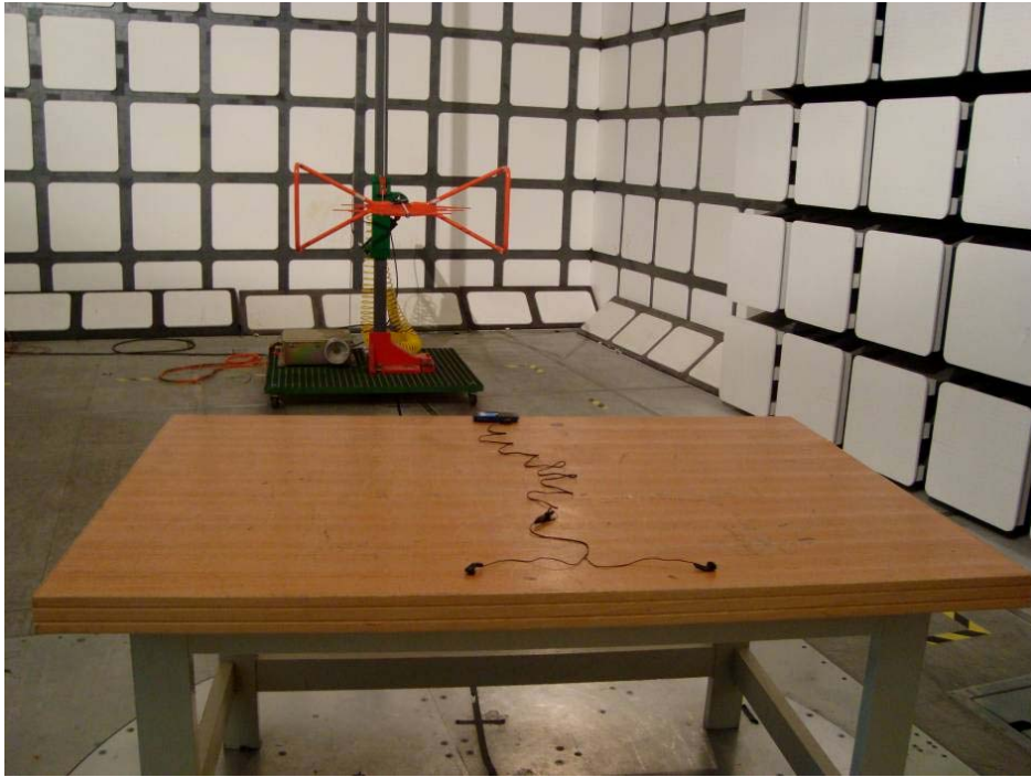
Radiated Emissions - Rear View (Media Playing mode)
