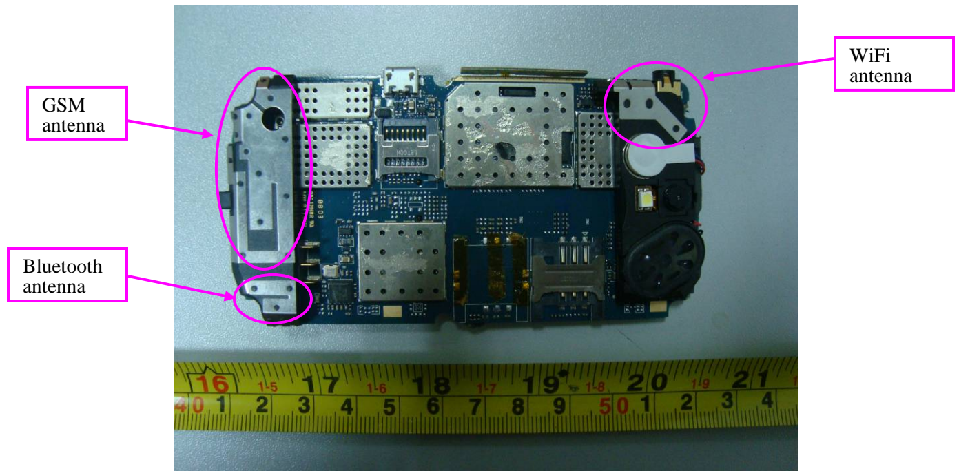
EUT – Main Board Top View
