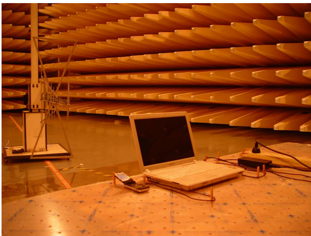
Pic 2 Radiated Emissions Test Setup
