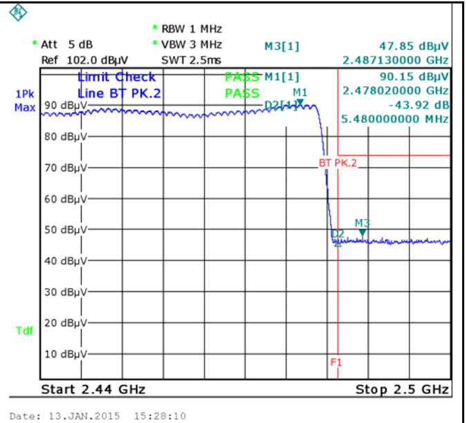
8DPSK-Hopping Right-PK
