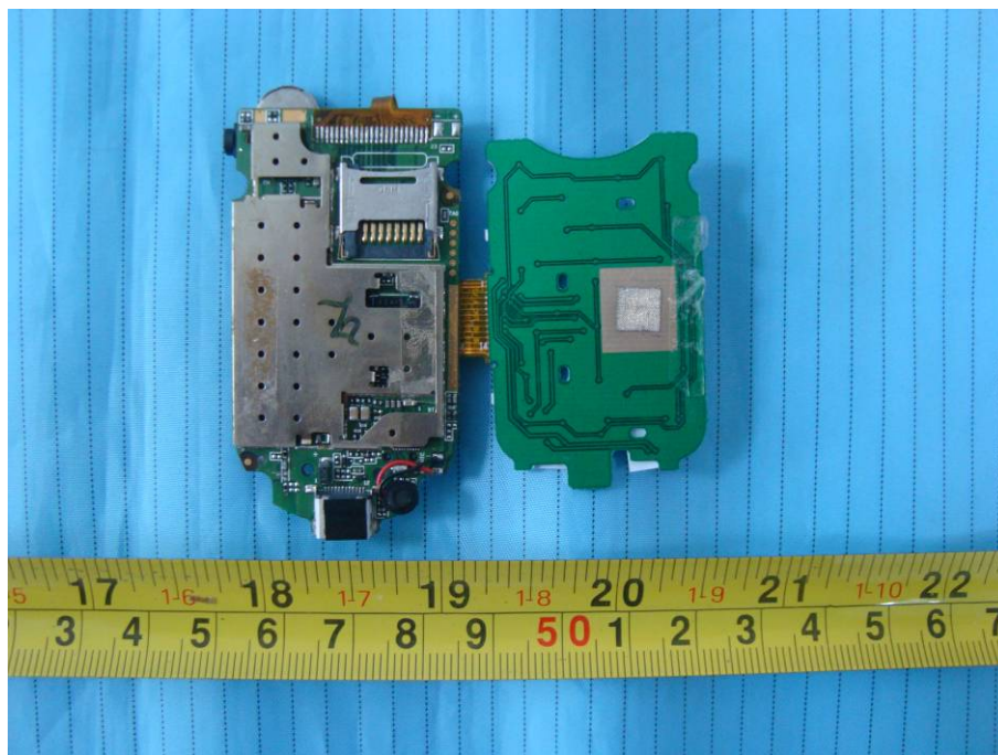
EUT – Main Board with Keyboard Cover off View
