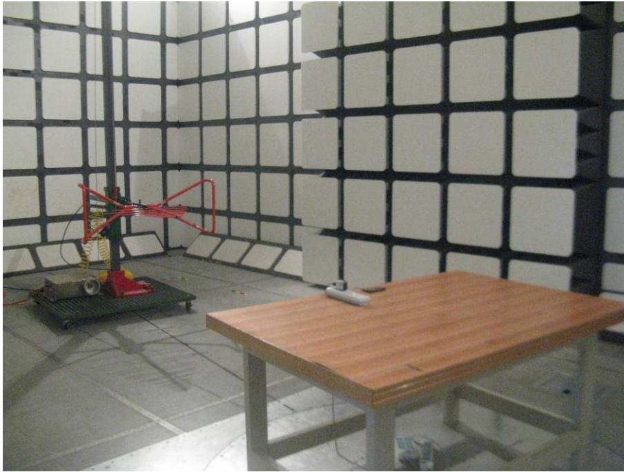
Radiated Emissions - Front View (Charging&multimedia playing)
