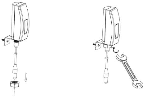
Figure 3-2: Sensor mounting
