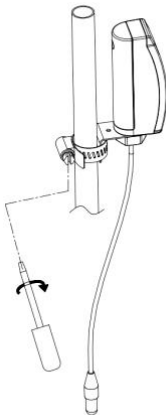
Figure 4: Sensor mounting to pole
