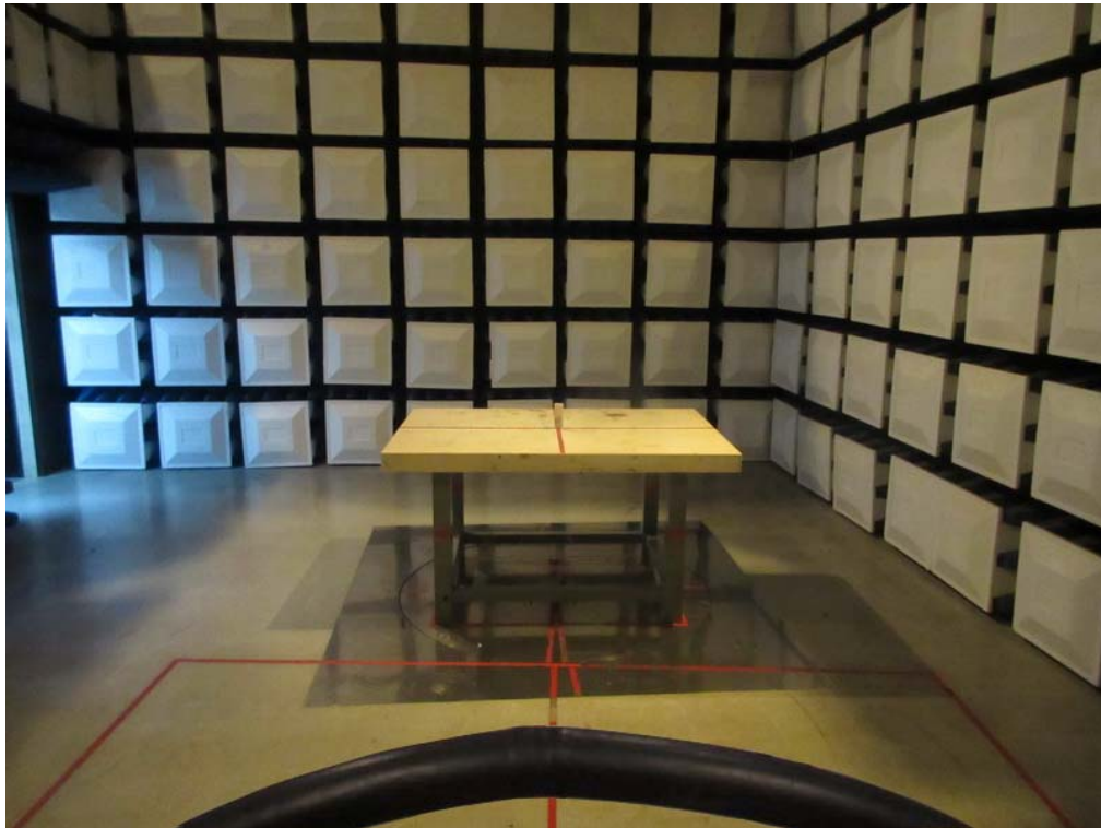
Radiated Measurement Photos 9KHz to 30MHz
