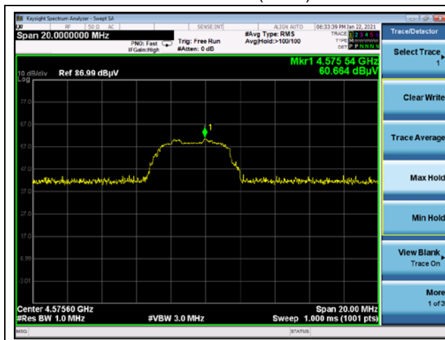
5 th harmonic (Peak)
