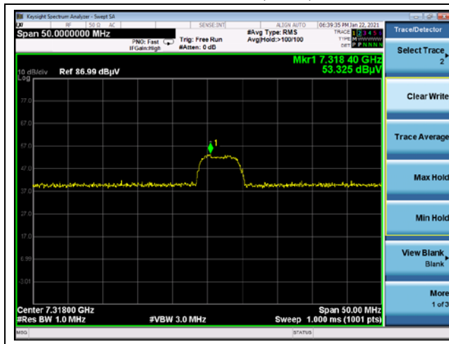
8 th harmonic (Peak)
