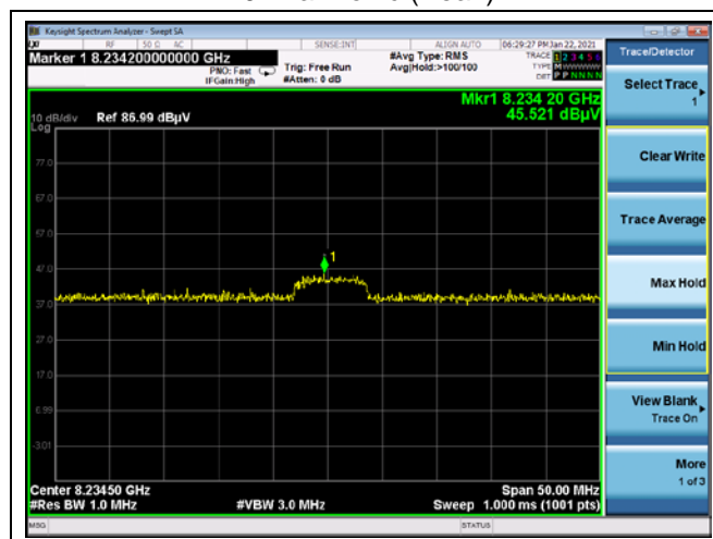
9 th harmonic (Peak)
