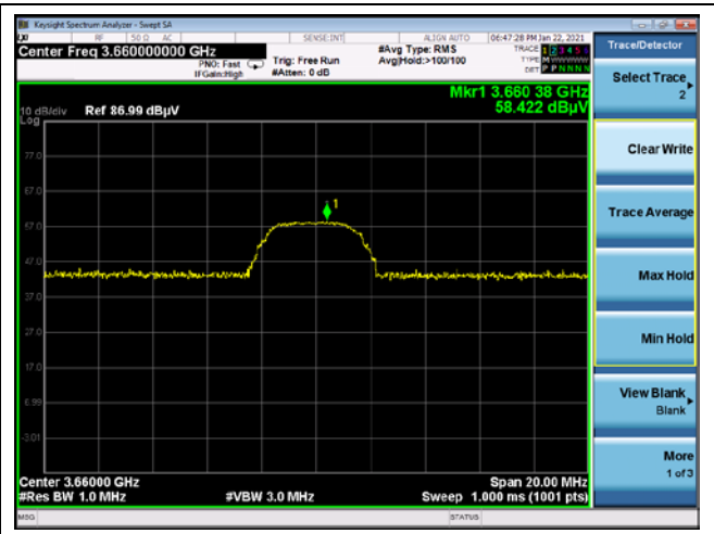
4 th harmonic (Peak)
