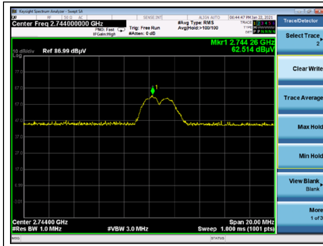
3 rd harmonic (Peak)
