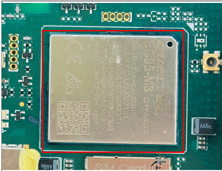
Top view of WWAN Module without Shielding
