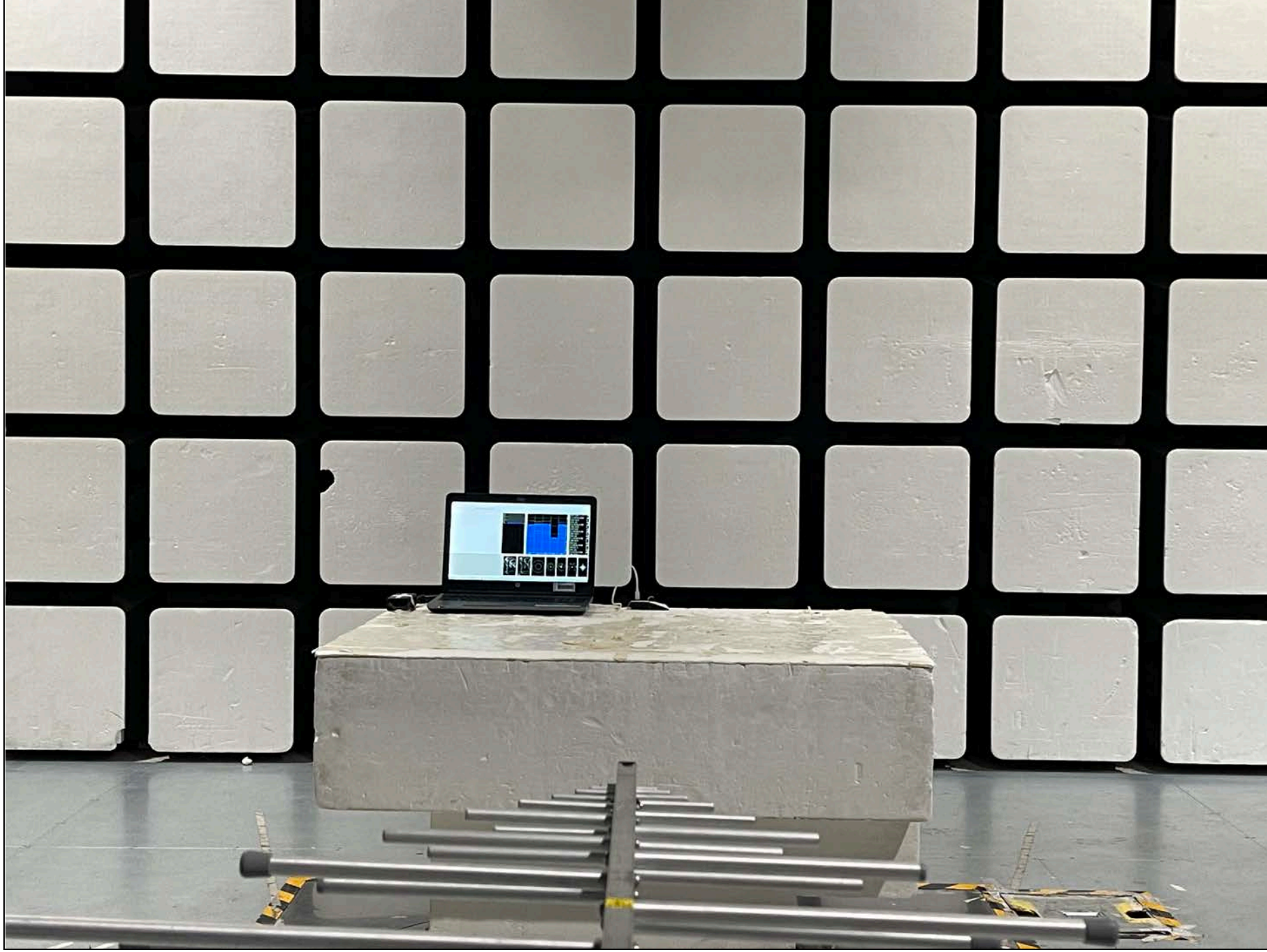
RE(Below 1 GHz)_Front
