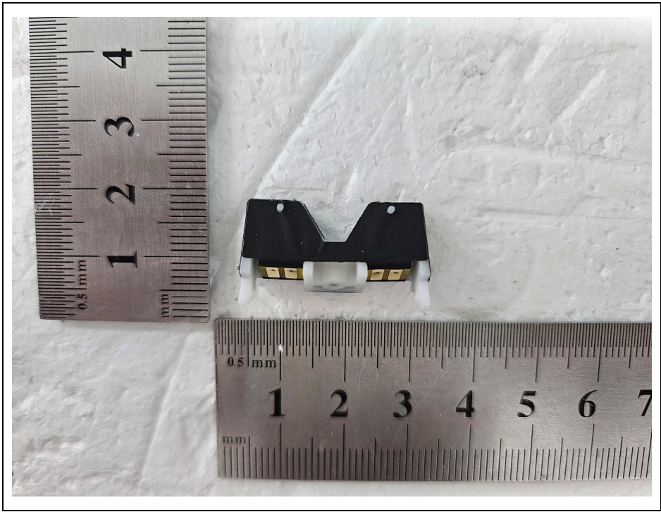
BT, WLAN Antenna
