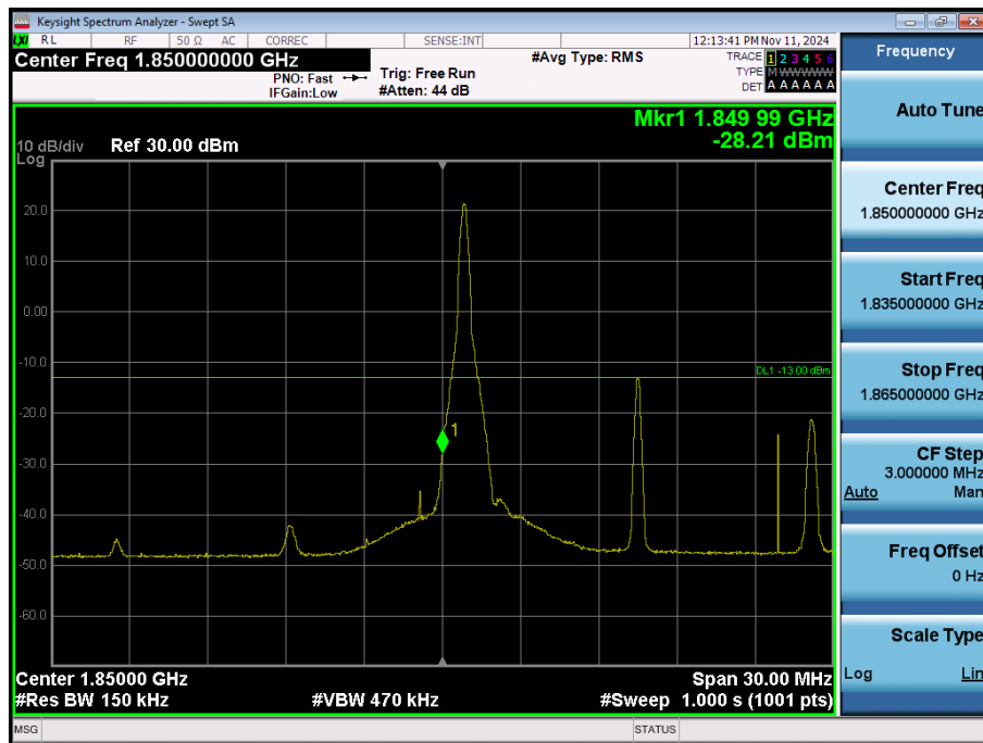
LTE Band 25 / 15MHz / QPSK - RB Size/Offset (1/0)
