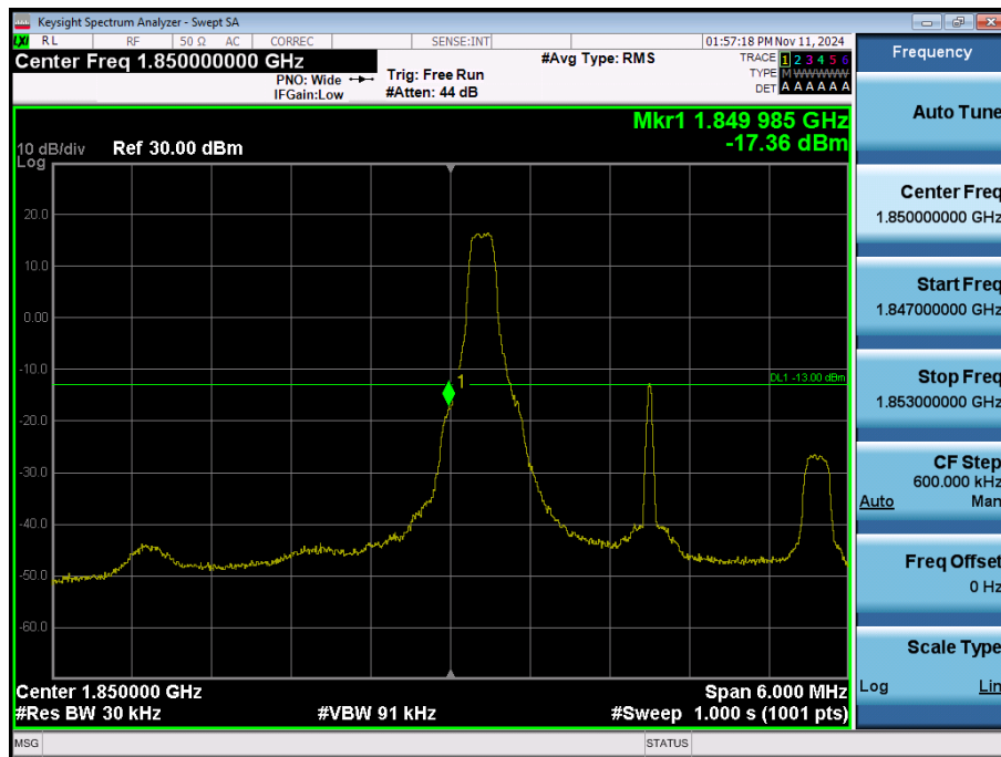
LTE Band 25 / 3MHz / QPSK - RB Size/Offset (8/0)
