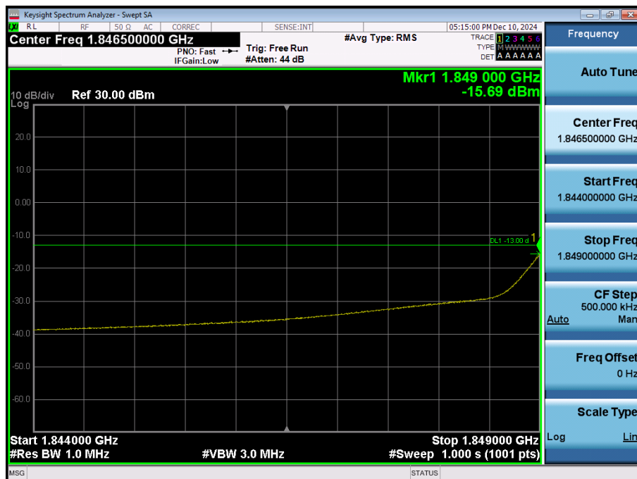
LTE Band 25 / 5MHz / 16QAM - RB Size/Offset (25/0)
