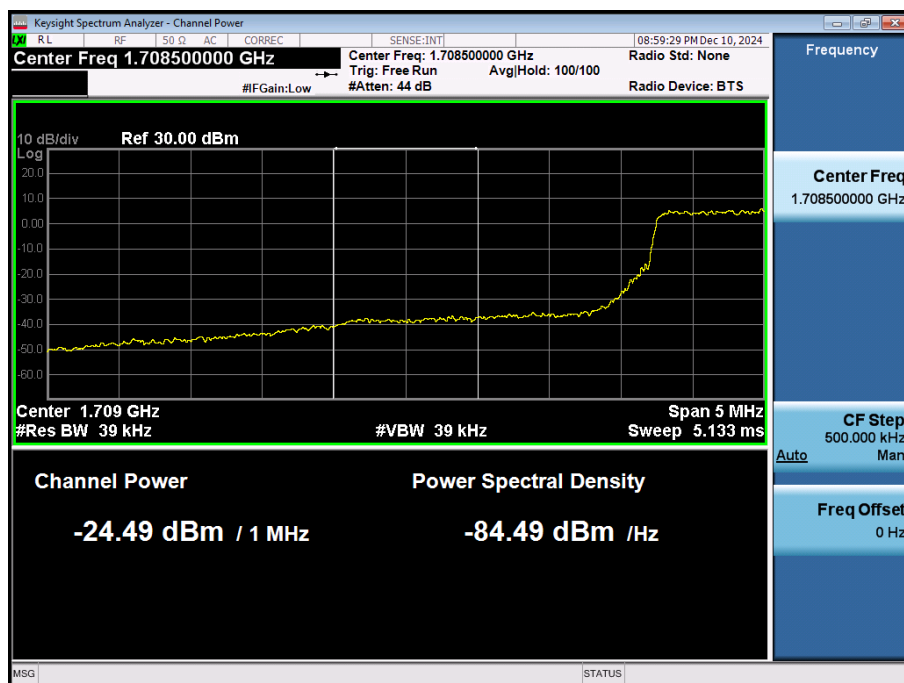
LTE Band 4 / 5MHz / QPSK - RB Size/Offset (12/6)
