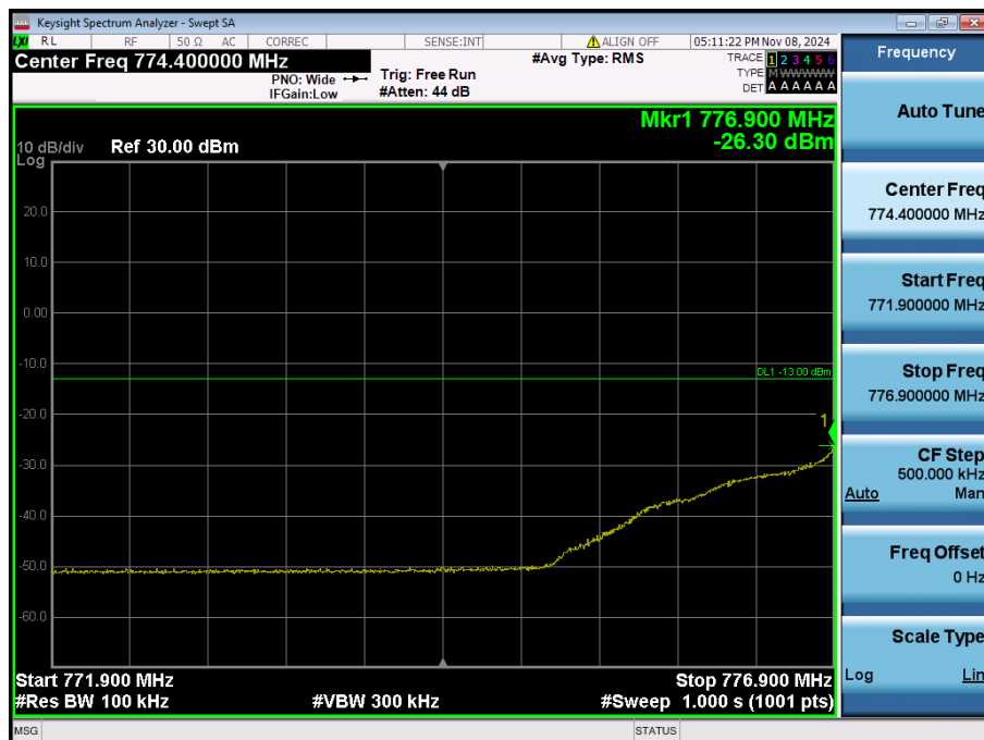
LTE Band 13 / 5MHz / QPSK - RB Size/Offset (12/6)
