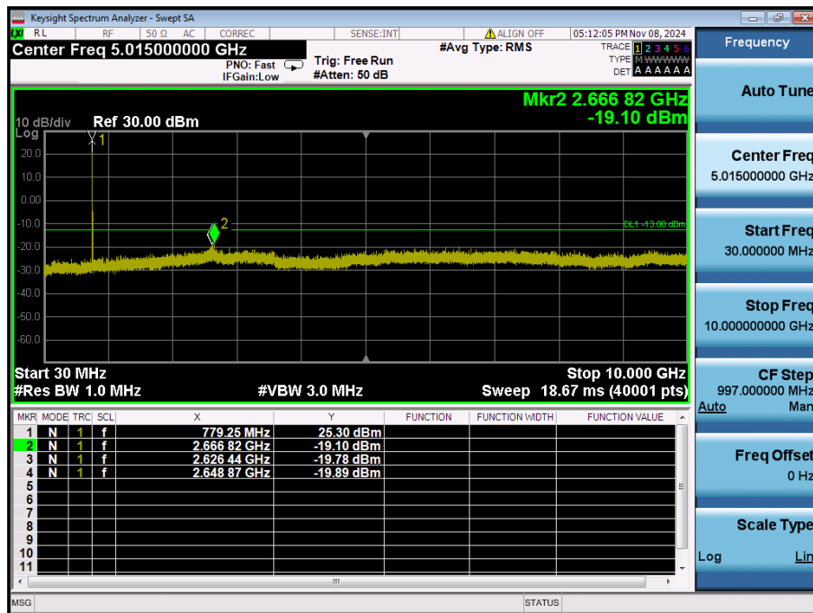
LTE Band 13 / 5MHz / QPSK - RB Size/Offset (12/6) - Low Channel
