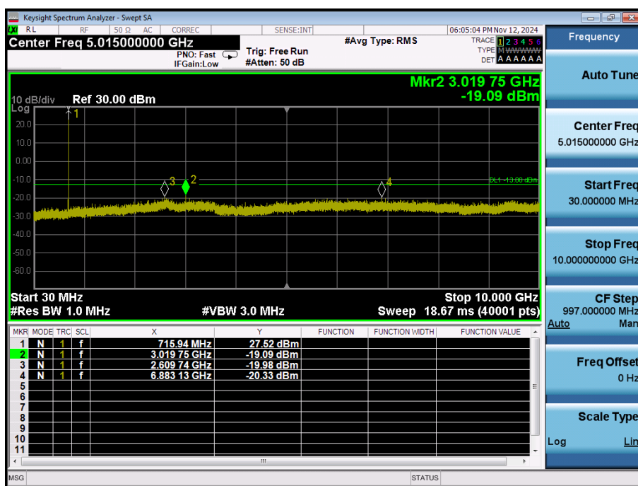
LTE Band 12 / 5MHz / QPSK - RB Size/Offset (1/24) - High Channel
