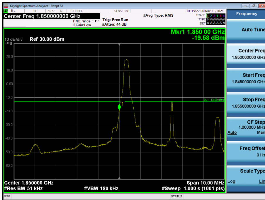
LTE Band 25 / 5MHz / QPSK - RB Size/Offset (1/0)
