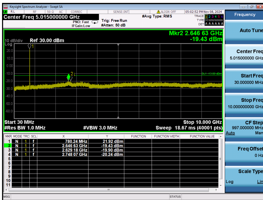
LTE Band 13 / 10MHz / QPSK - RB Size/Offset (50/0) - Low Channel
