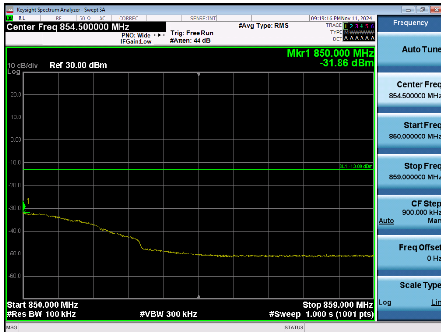
LTE Band 26 / 10MHz / 16QAM - RB Size/Offset (25/25)
