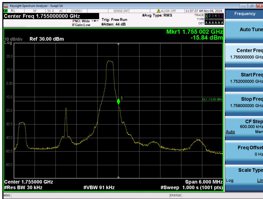
LTE Band 4 / 3MHz / QPSK - RB Size/Offset (8/7)
