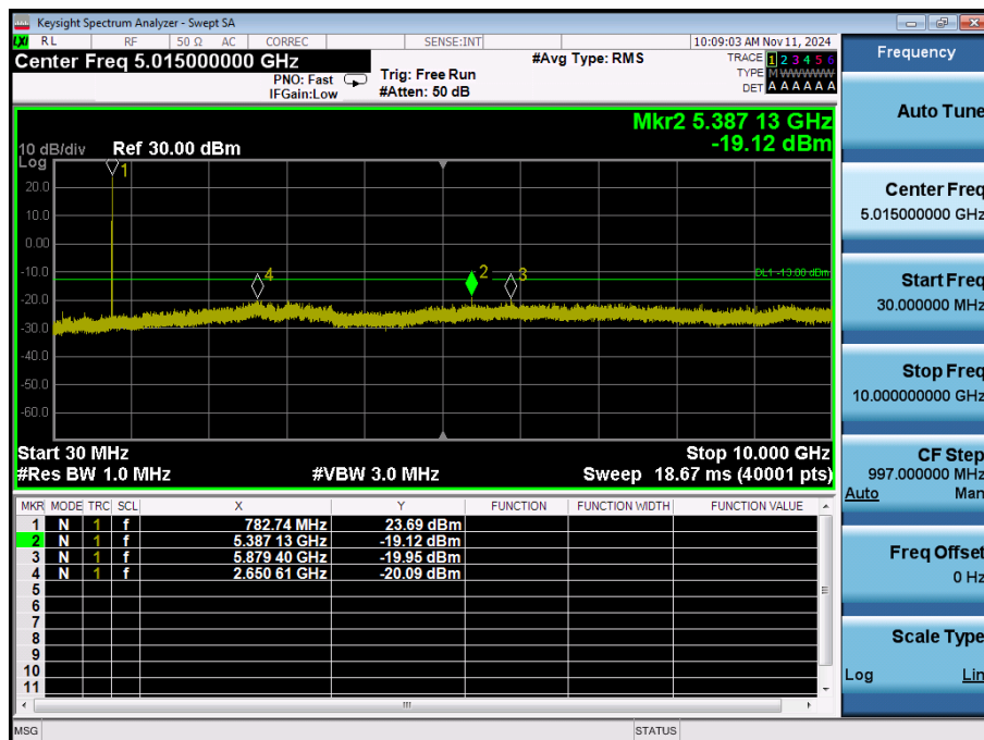
LTE Band 13 / 5MHz / 16QAM - RB Size/Offset (12/0) - High Channel
