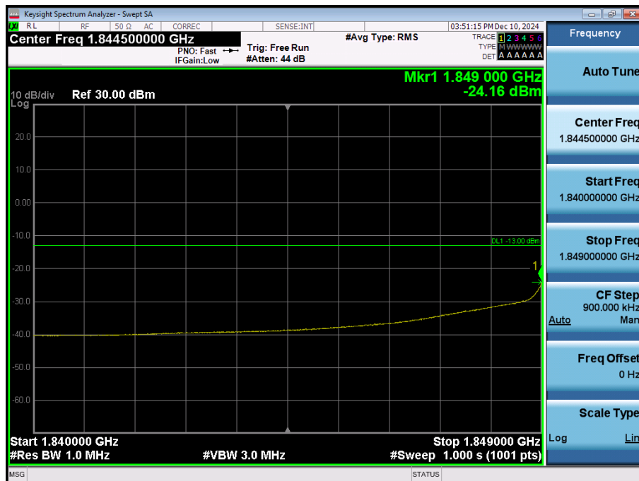
LTE Band 25 / 10MHz / QPSK - RB Size/Offset (25/12)
