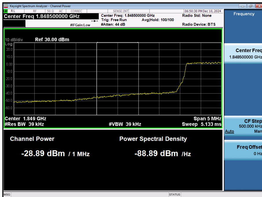
LTE Band 25 / 3MHz / 16QAM - RB Size/Offset (15/0)
