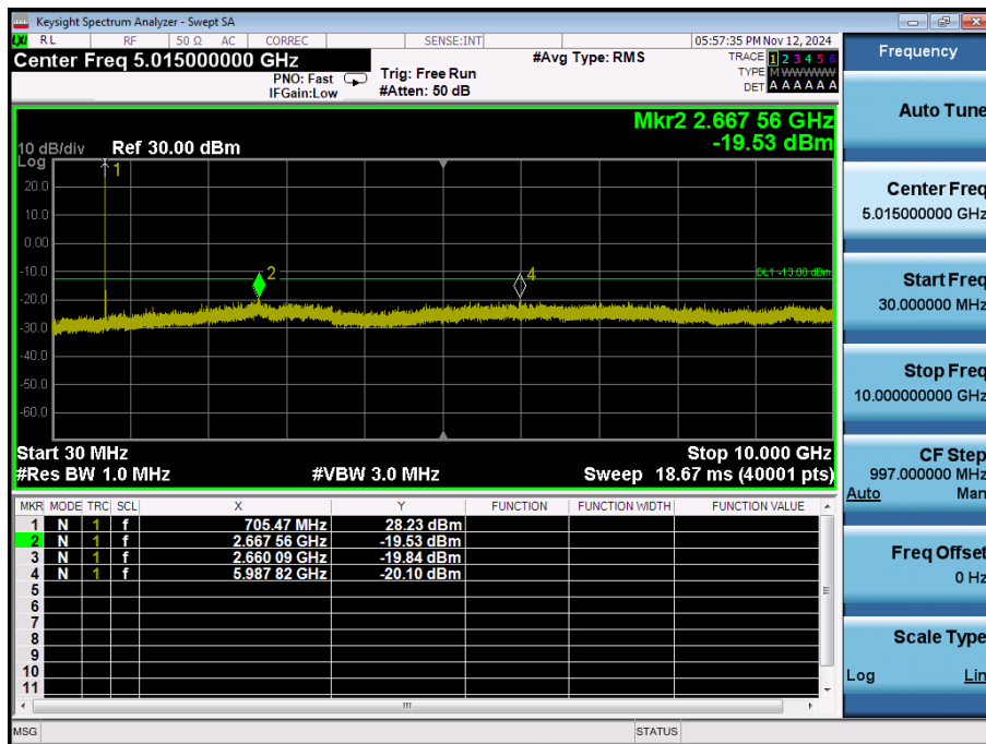
LTE Band 12 / 5MHz / QPSK - RB Size/Offset (1/0) - Mid Channel
