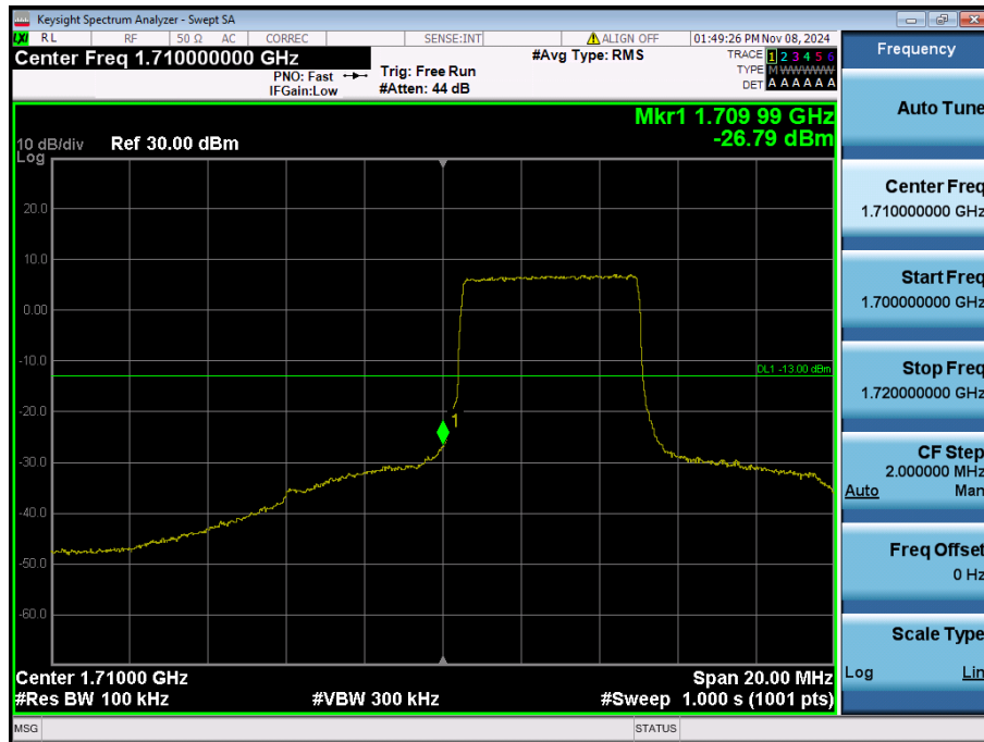
LTE Band 4 / 10MHz / 16QAM - RB Size/Offset (25/12)
