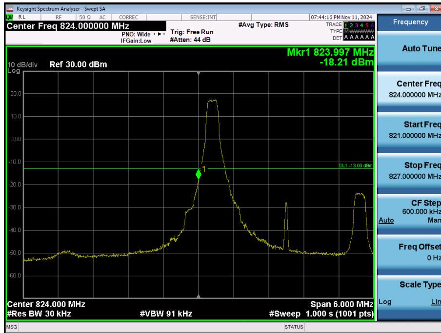
LTE Band 26 / 3MHz / QPSK - RB Size/Offset (8/0)
