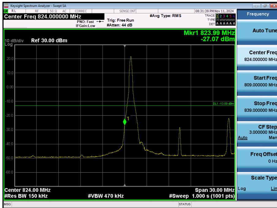
LTE Band 26 / 15MHz / 16QAM - RB Size/Offset (1/0)
