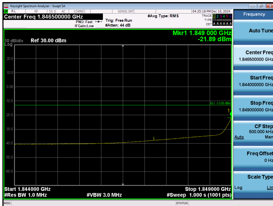
LTE Band 25 / 1.4MHz / QPSK - RB Size/Offset (1/2)
