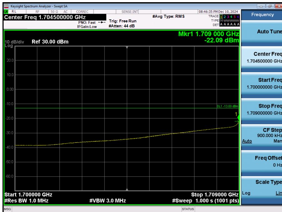
LTE Band 4 / 10MHz / QPSK - RB Size/Offset (25/12)
