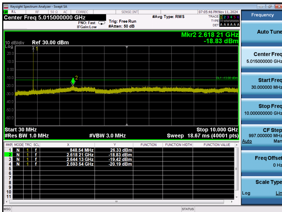
LTE Band 26 / 10MHz / QPSK - RB Size/Offset (1/49) - High Channel
