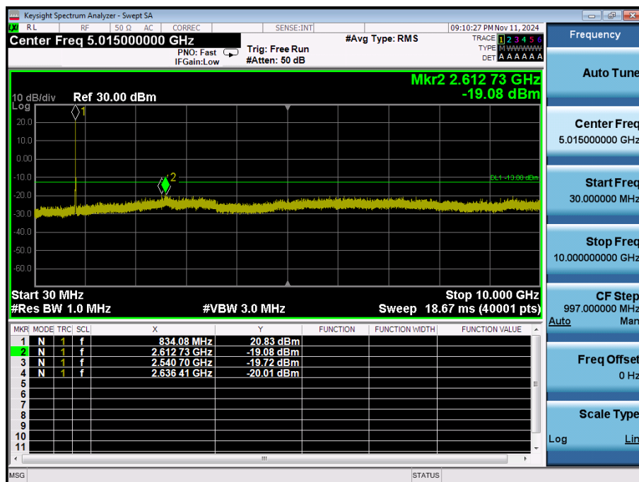
LTE Band 26 / 10MHz / 16QAM - RB Size/Offset (50/0) - Mid Channel
