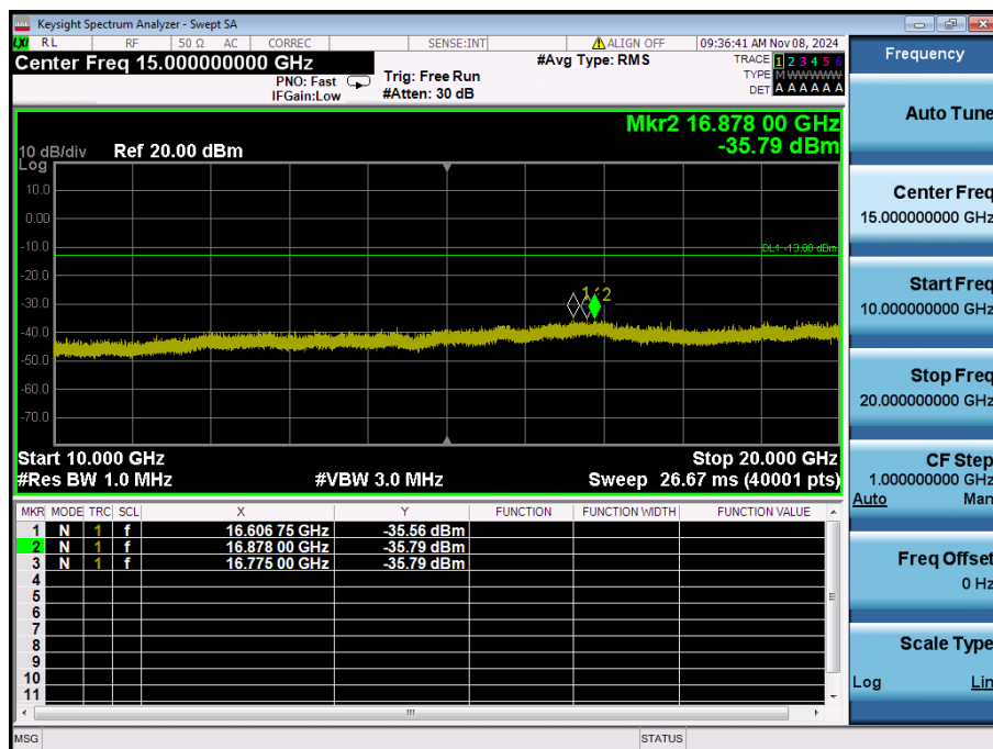
LTE Band 4 / 20MHz / QPSK - RB Size/Offset (100/0) - Mid Channel
