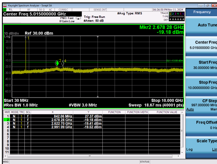
LTE Band 26 / 15MHz / QPSK - RB Size/Offset (1/036) - High Channel
