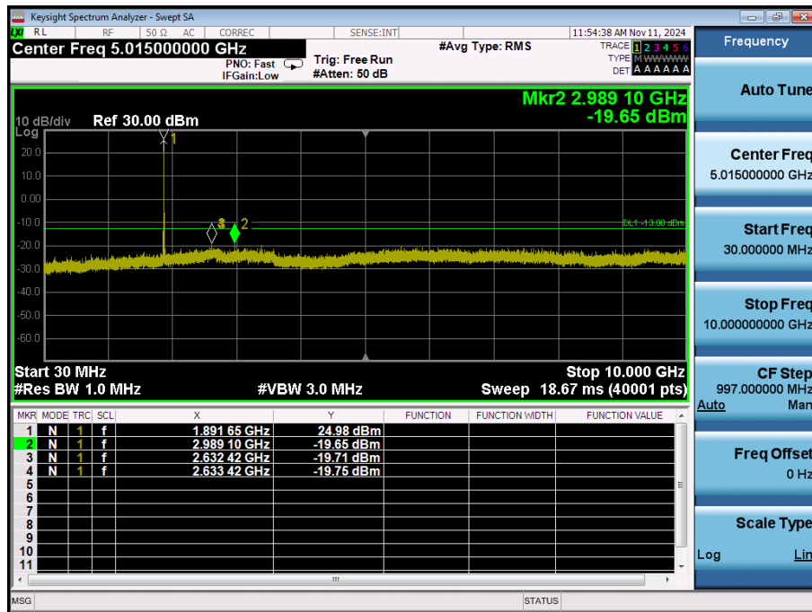
LTE Band 25 / 20MHz / QPSK - RB Size/Offset (1/99) - Mid Channel
