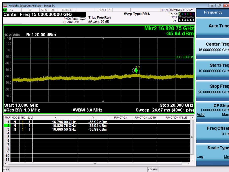
LTE Band 25 / 20MHz / 16QAM - RB Size/Offset (50/50) - High Channel
