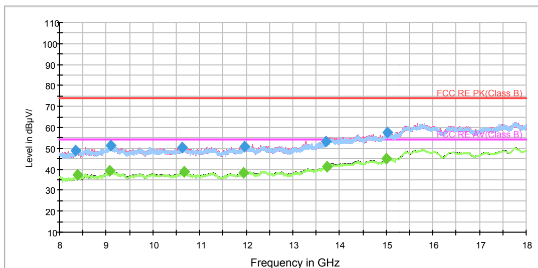
Radiated Emission from 8GHz to 18GHz
