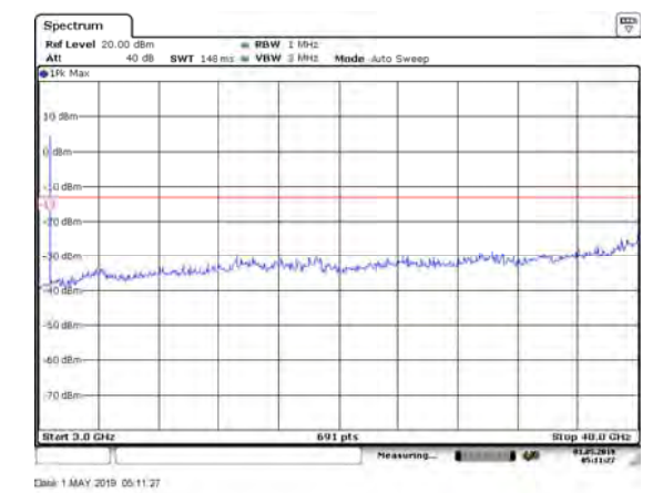
LTE Band 43 5MHz CH Middle 3GHz~40GHz
