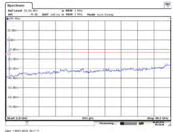
LTE Band 43 5MHz CH Low 3GHz~40GHz
