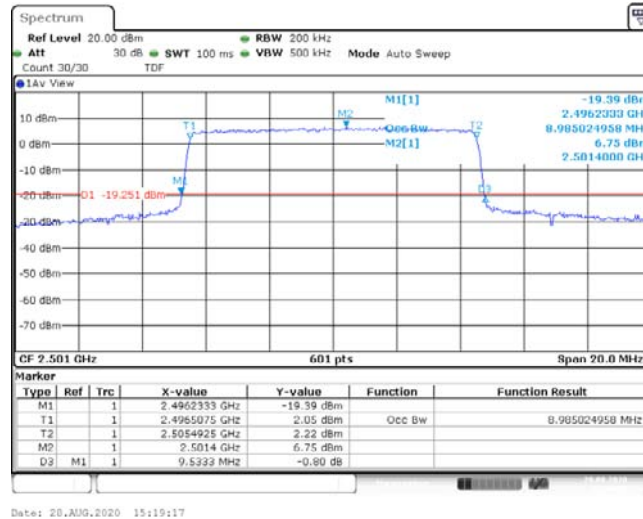
Band41-10MHz-16QAM-39700-50RB#0-8.985-9.533-PASS
