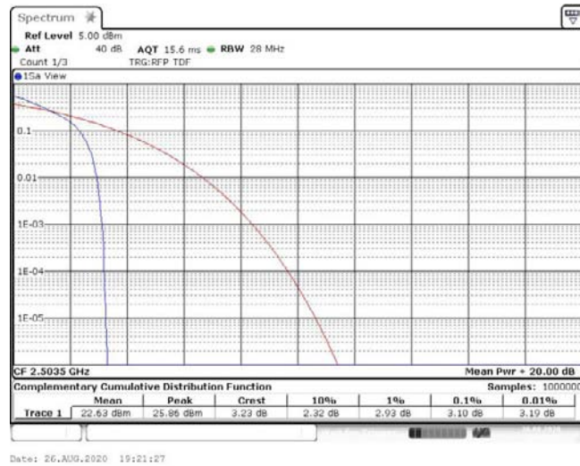
Band41-15MHz-QPSK-39725-1RB#0-3.10-13-PASS
