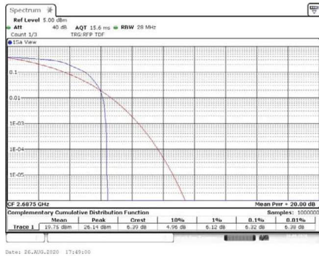
Band41-5MHz-QPSK-41565-25RB#0-6.32-13-PASS
