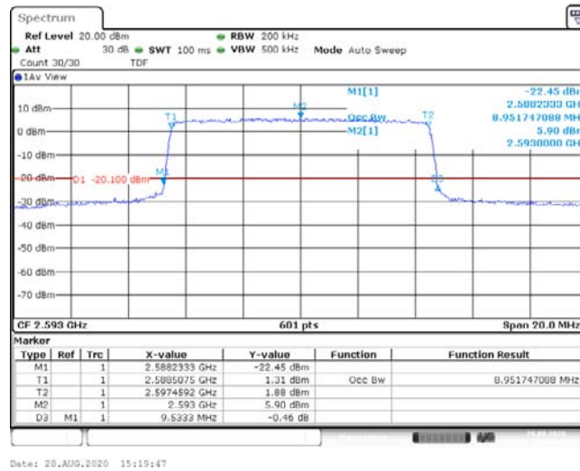
Band41-10MHz-16QAM-40620-50RB#0-8.952-9.533-PASS
