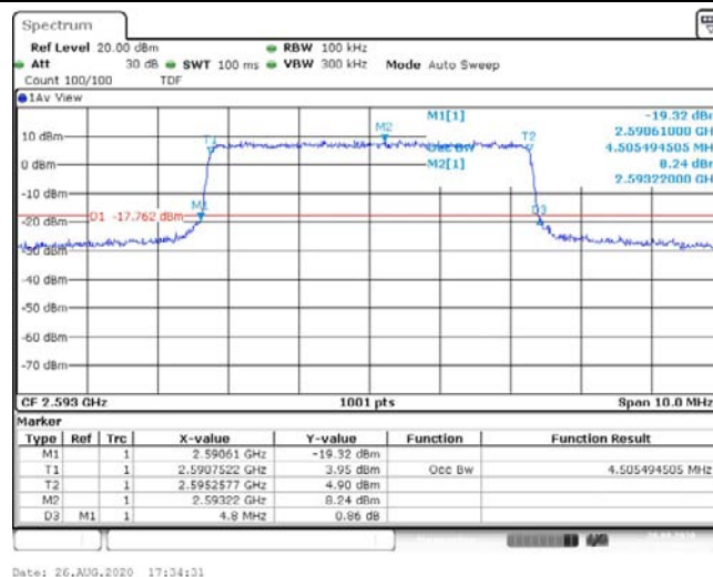
Band41-5MHz-QPSK-40620-25RB#0-4.505-4.800-PASS
