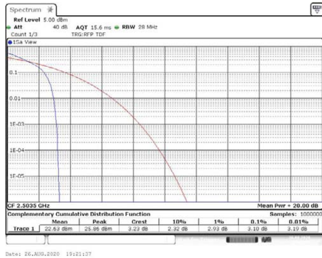
Band41-15MHz-16QAM-39725-1RB#0-3.10-13-PASS
