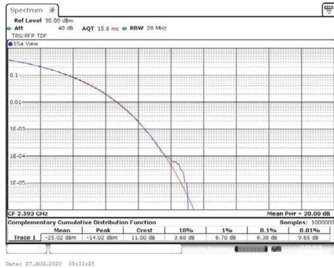
Band41-20MHz-16QAM-40620-100RB#0-8.38-13-PASS
