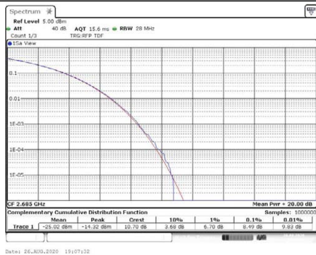
Band41-10MHz-16QAM-41540-1RB#0-8.49-13-PASS
