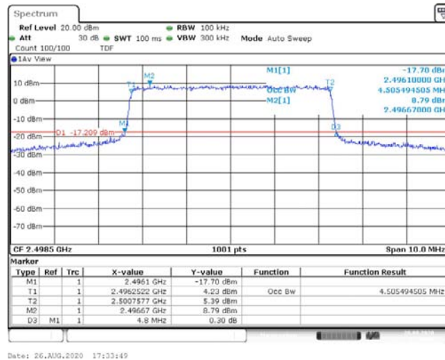
Band41-5MHz-QPSK-39675-25RB#0-4.505-4.800-PASS
