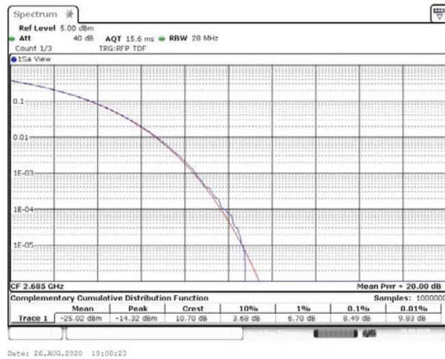
Band41-10MHz-16QAM-41540-50RB#0-8.49-13-PASS
