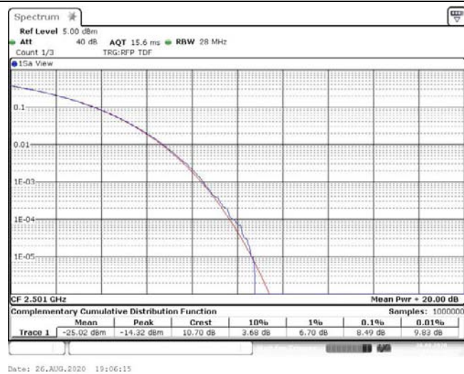
Band41-10MHz-16QAM-39700-50RB#0-8.49-13-PASS
