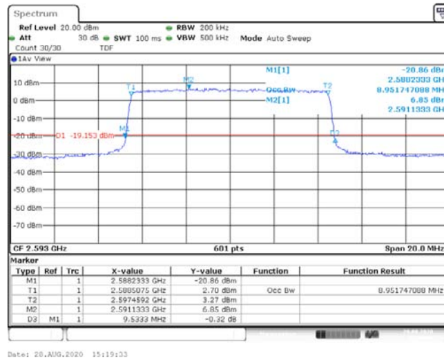
Band41-10MHz-QPSK-40620-50RB#0-8.952-9.533-PASS
