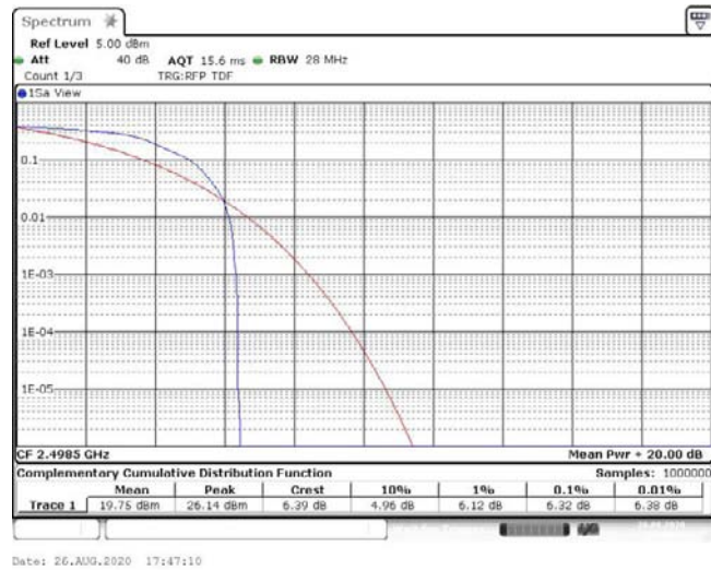
Band41-5MHz-16QAM-39675-1RB#0-6.32-13-PASS
