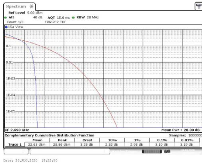
Band41-15MHz-16QAM-40620-1RB#0-3.10-13-PASS
