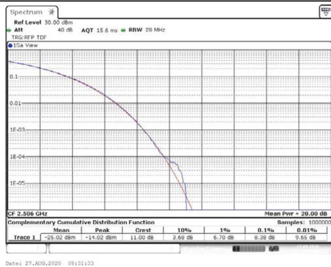
Band41-20MHz-QPSK-39750-100RB#0-8.38-13-PASS
