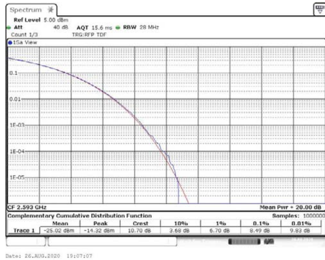
Band41-10MHz-16QAM-40620-50RB#0-8.49-13-PASS
