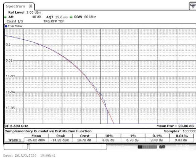
Band41-10MHz-16QAM-40620-1RB#0-8.49-13-PASS
