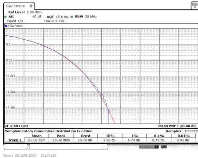
Band41-10MHz-16QAM-39700-1RB#0-8.49-13-PASS
