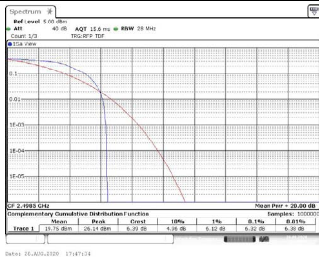
Band41-5MHz-16QAM-39675-25RB#0-6.32-13-PASS
