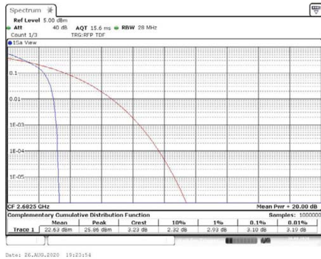
Band41-15MHz-QPSK-41515-75RB#0-3.10-13-PASS
