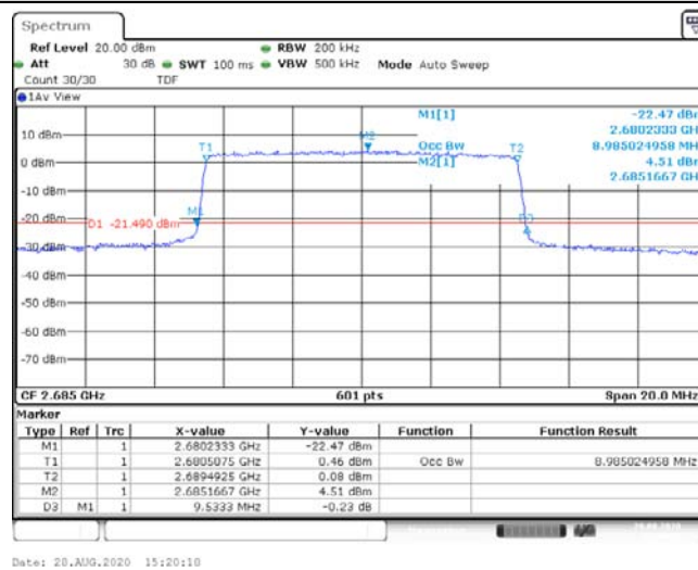
Band41-10MHz-16QAM-41540-50RB#0-8.985-9.533-PASS
