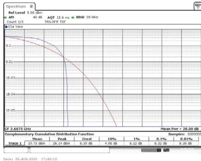
Band41-5MHz-16QAM-41565-25RB#0-6.32-13-PASS
