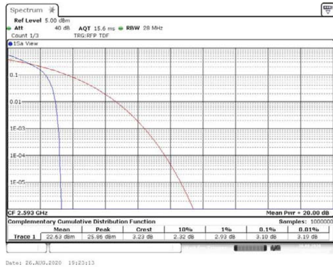
Band41-15MHz-16QAM-40620-75RB#0-3.10-13-PASS
