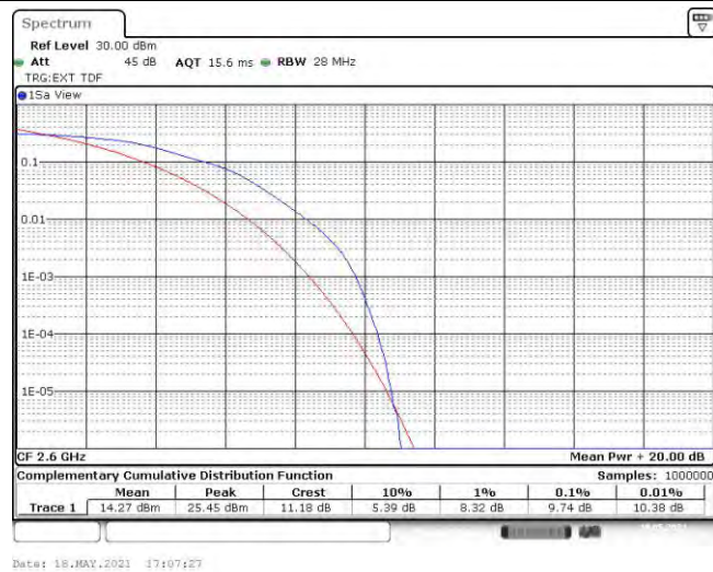
Band41-10MHz-16QAM-41540-50RB#0
