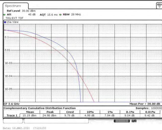
Band41-15MHz-QPSK-41515-75RB#0
