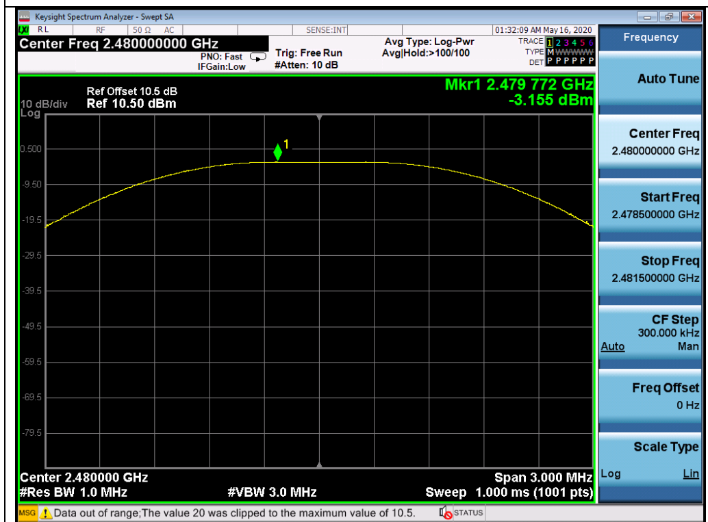
BLE-2480MHz
