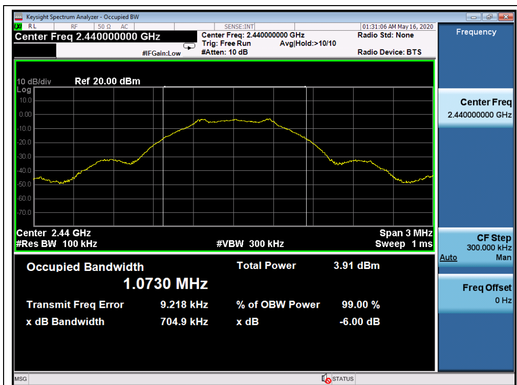
BLE-2440MHz
