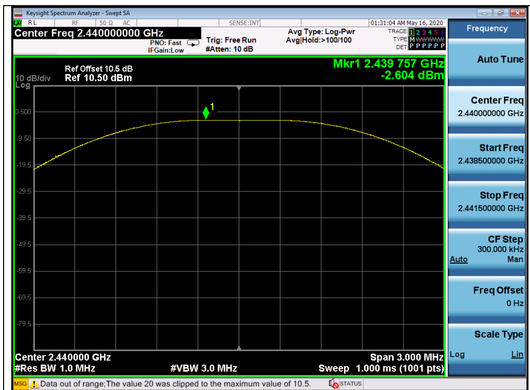
BLE-2440MHz
