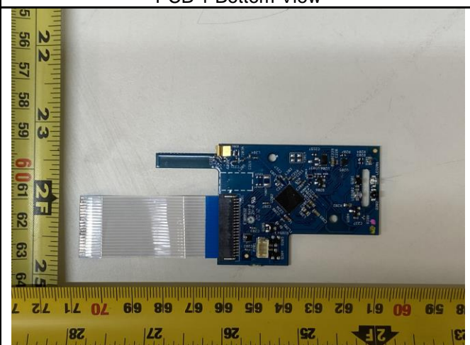
Main Circuit Board inside Internal Enclosure
