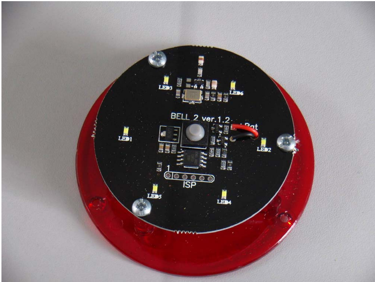
Figure 1 –Front view.
