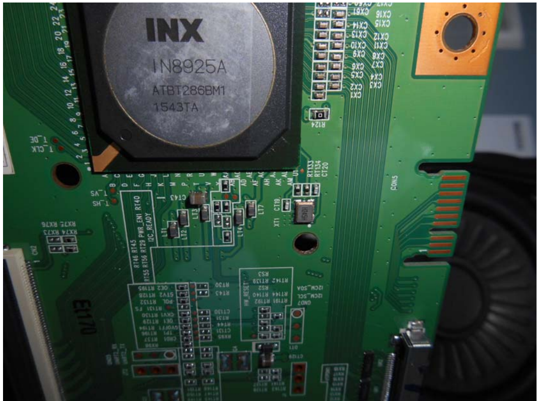
FIGURE 21 LED LCD TV (M/N: LC-75N8000U) CHIP AND CRYSTAL ON PANEL BOARD
