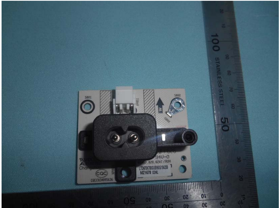
FIGURE 5 LED LCD TV (M/N: LC-75N8000U) AC BOARD (COMPONENT SIDE)
