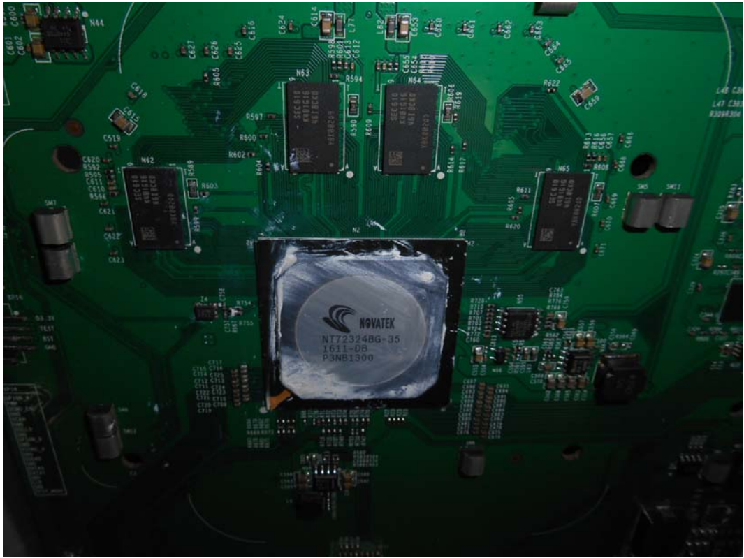
FIGURE 10 LED LCD TV (M/N: LC-75N8000U) CHIP#2 AND CRYSTAL #2 ON MAIN BOARD
