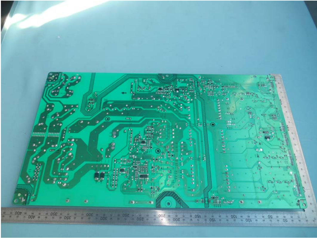
FIGURE 4 LED LCD TV (M/N: LC-75N8000U) POWER BOARD (SOLDERED SIDE)
