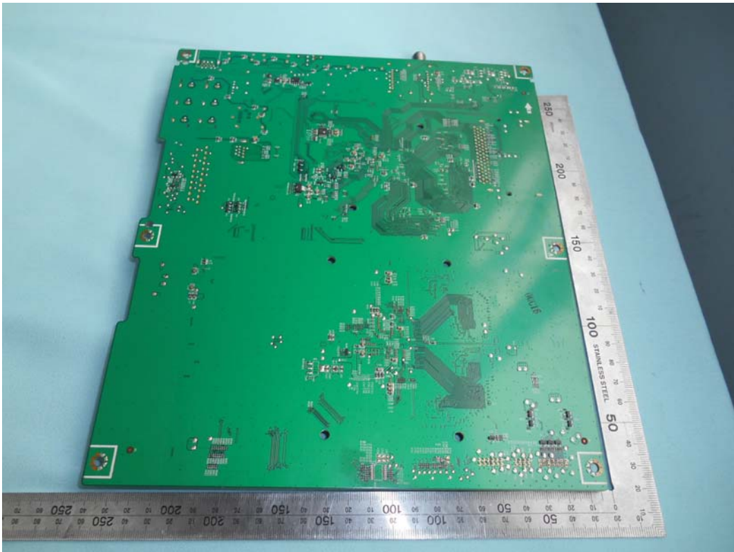
FIGURE 8 LED LCD TV (M/N: LC-75N8000U) MAIN BOARD (SOLDERED SIDE)
