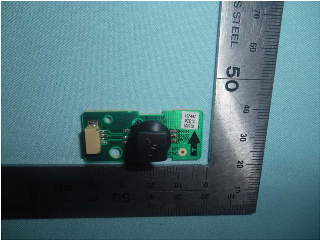
FIGURE 14 LED LCD TV (M/N: LC-75N8000U) KEY BOARD (COMPONENT SIDE)
