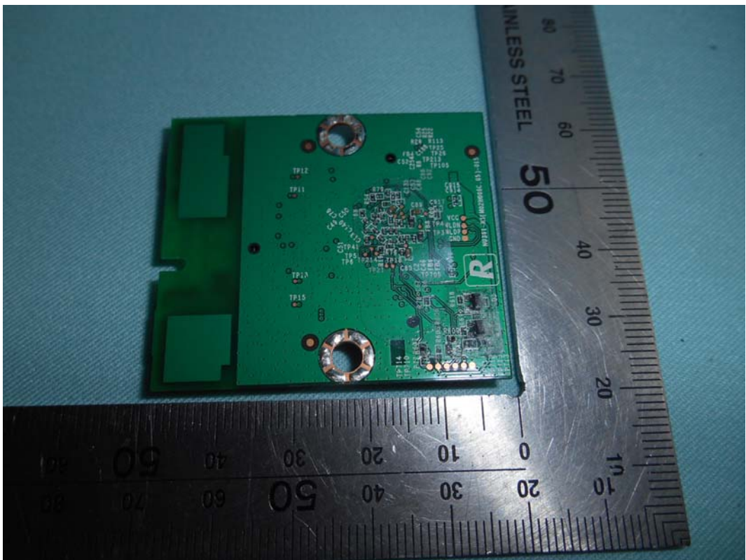
FIGURE 17 LED LCD TV (M/N: LC-75N8000U) RF BOARD (SOLDERED SIDE)
