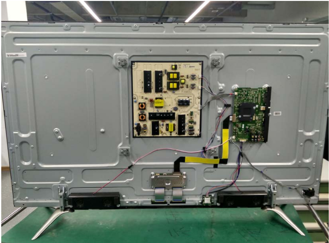
FIGURE 1 LED LCD TV (M/N: LTDN65K550GUWUS) COVER REMOVED
