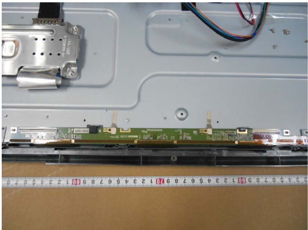
FIGURE 28 LED LCD TV (M/N: LTDN65K550GUWUS) DEBUG #2
