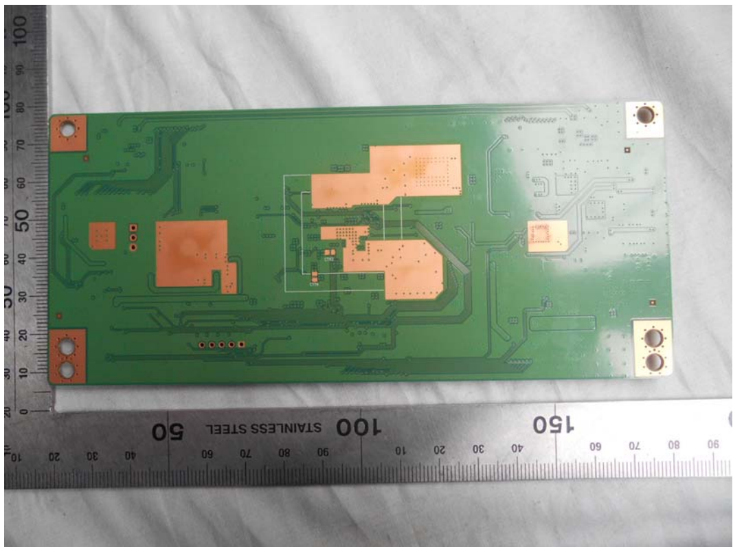
FIGURE 11 LED LCD TV (M/N: LTDN65K550GUWUS) PANEL BOARD (SOLDERED SIDE)
