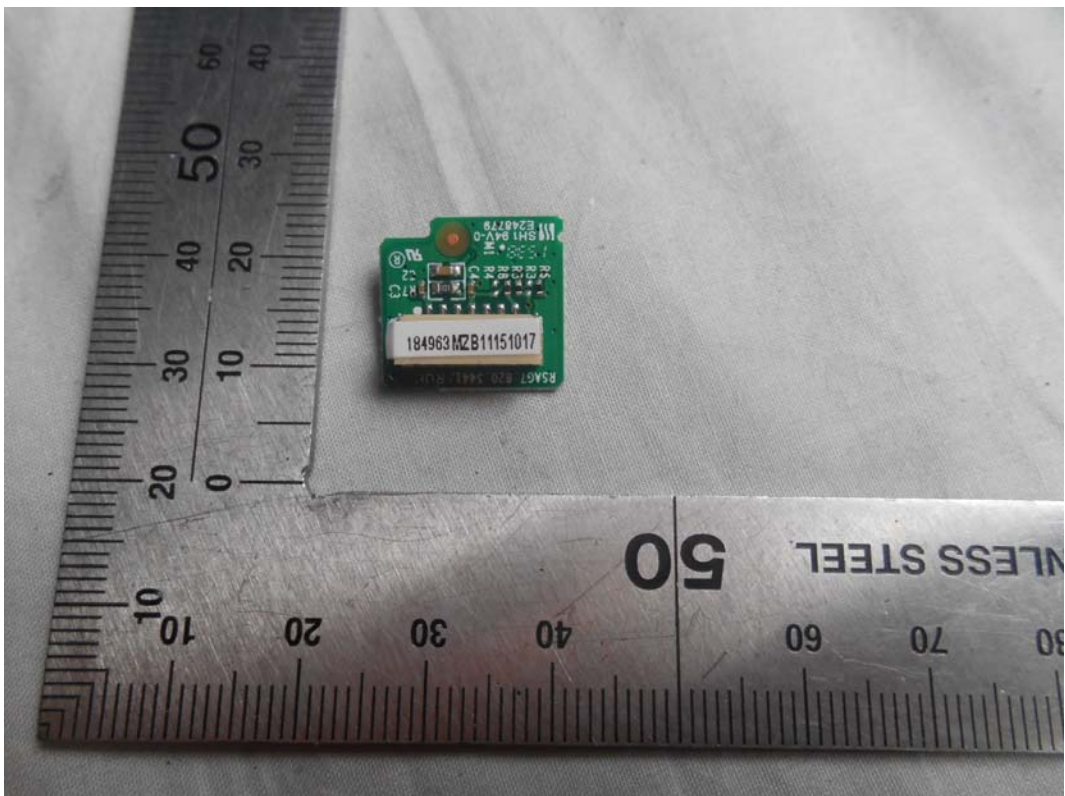
FIGURE 20 LED LCD TV (M/N: LTDN65K550GUWUS) IR BOARD (SOLDERED SIDE)
