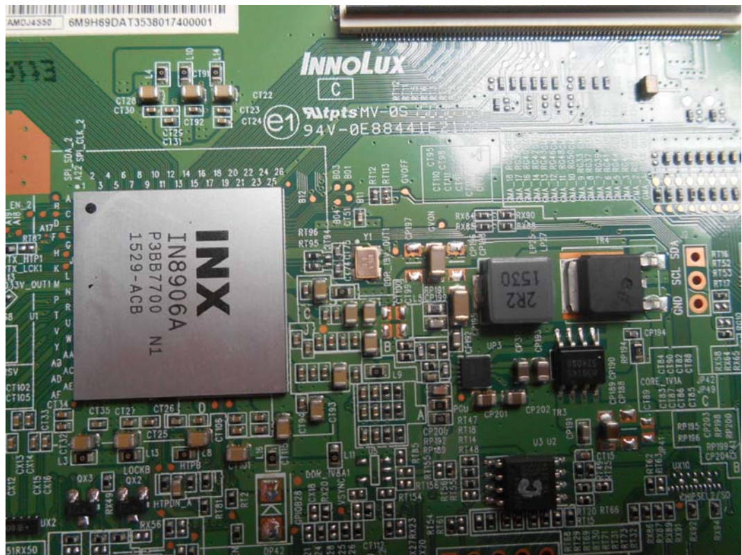
FIGURE 12 LED LCD TV (M/N: LTDN65K550GUWUS) CHIP & CRYSTAL ON PANEL BOARD
