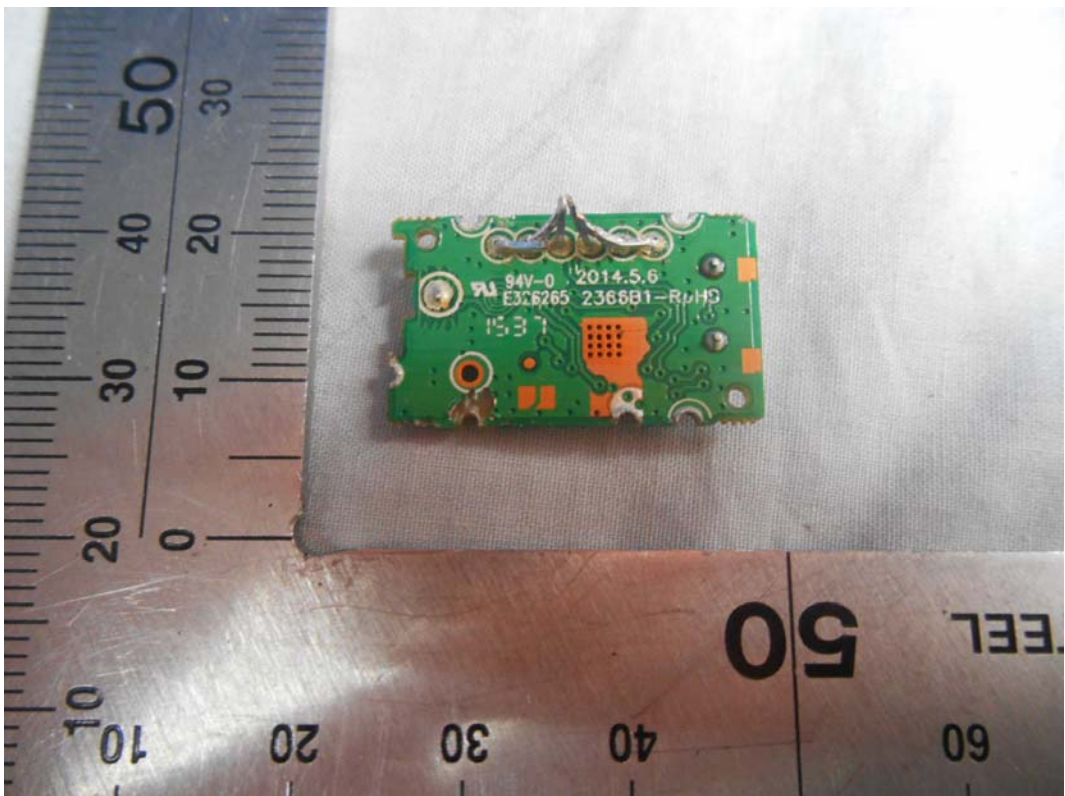
FIGURE 9 LED LCD TV (M/N: LTDN65K550GUWUS) TUNER BOARD (SOLDERED SIDE)
