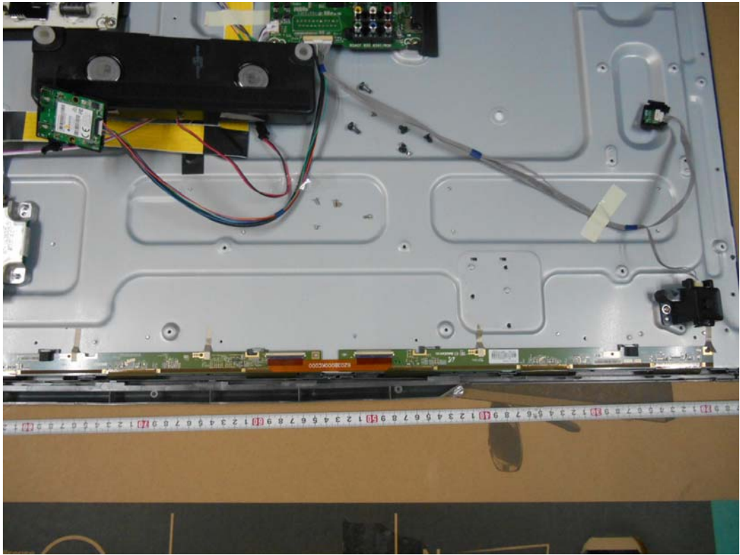
FIGURE 21 LED LCD TV (M/N: LTDN65K550GUWUS) SIGNAL BOARD#1 (COMPONENT SIDE)
