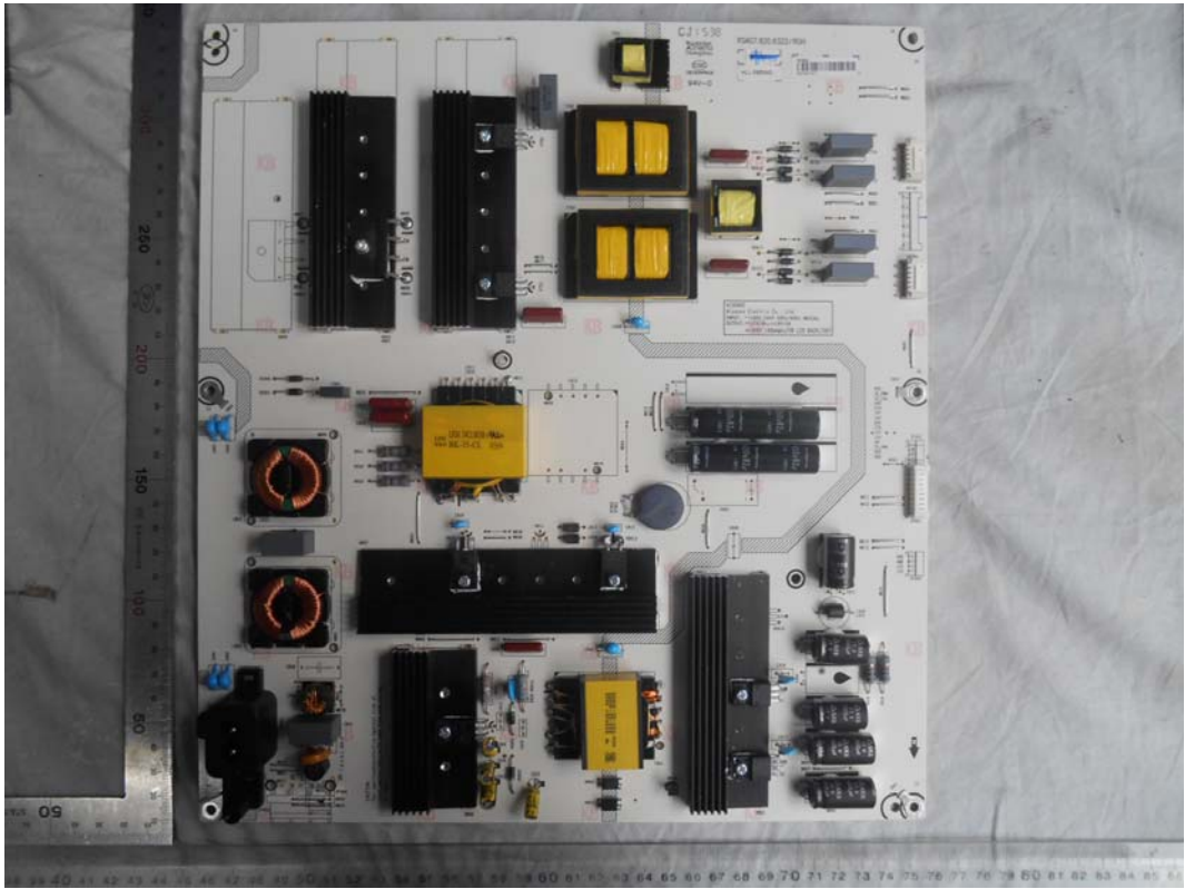
FIGURE 17 LED LCD TV (M/N: LTDN65K550GUWUS) POWER BOARD (COMPONENT SIDE)
