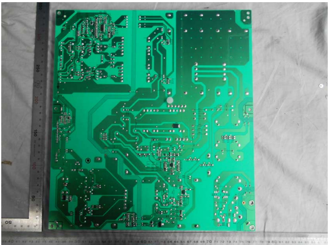
FIGURE 18 LED LCD TV (M/N: LTDN65K550GUWUS) POWER BOARD (SOLDERED SIDE)
