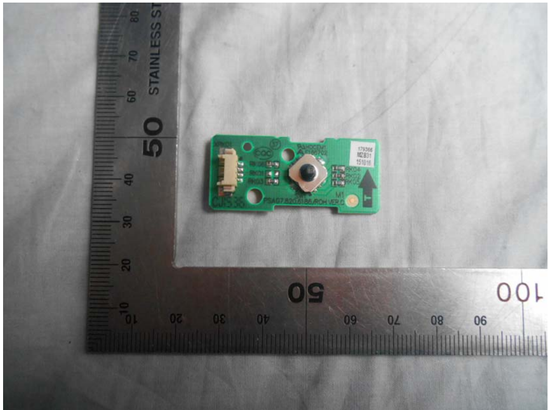
FIGURE 25 LED LCD TV (M/N: LTDN65K550GUWUS) KEY BOARD (COMPONENT SIDE)
