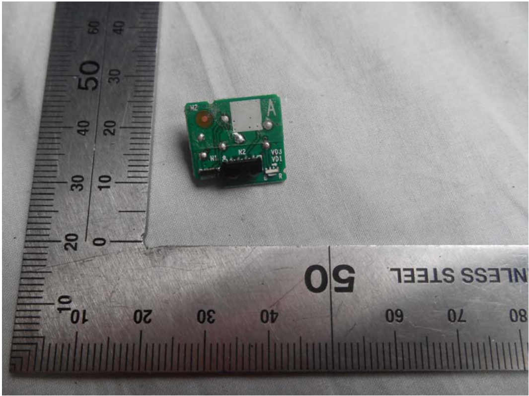
FIGURE 19 LED LCD TV (M/N: LTDN65K550GUWUS) IR BOARD (COMPONENT SIDE)
