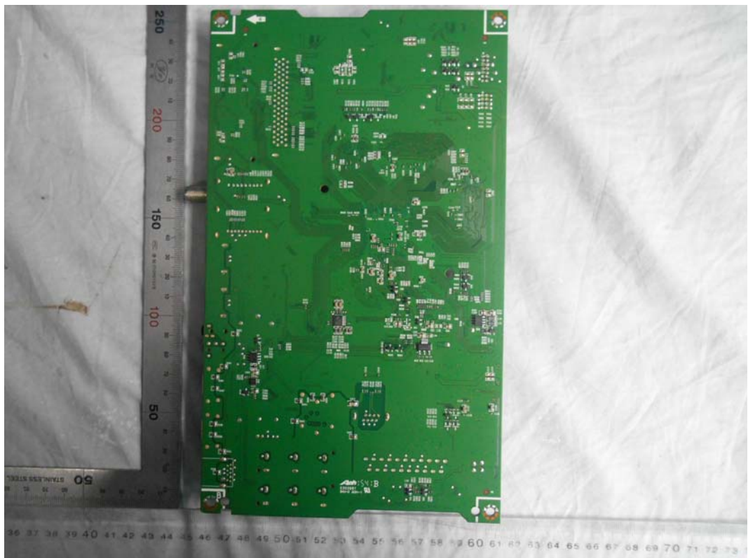
FIGURE 5 LED LCD TV (M/N: LTDN65K550GUWUS) MAIN BOARD (SOLDERED SIDE)
