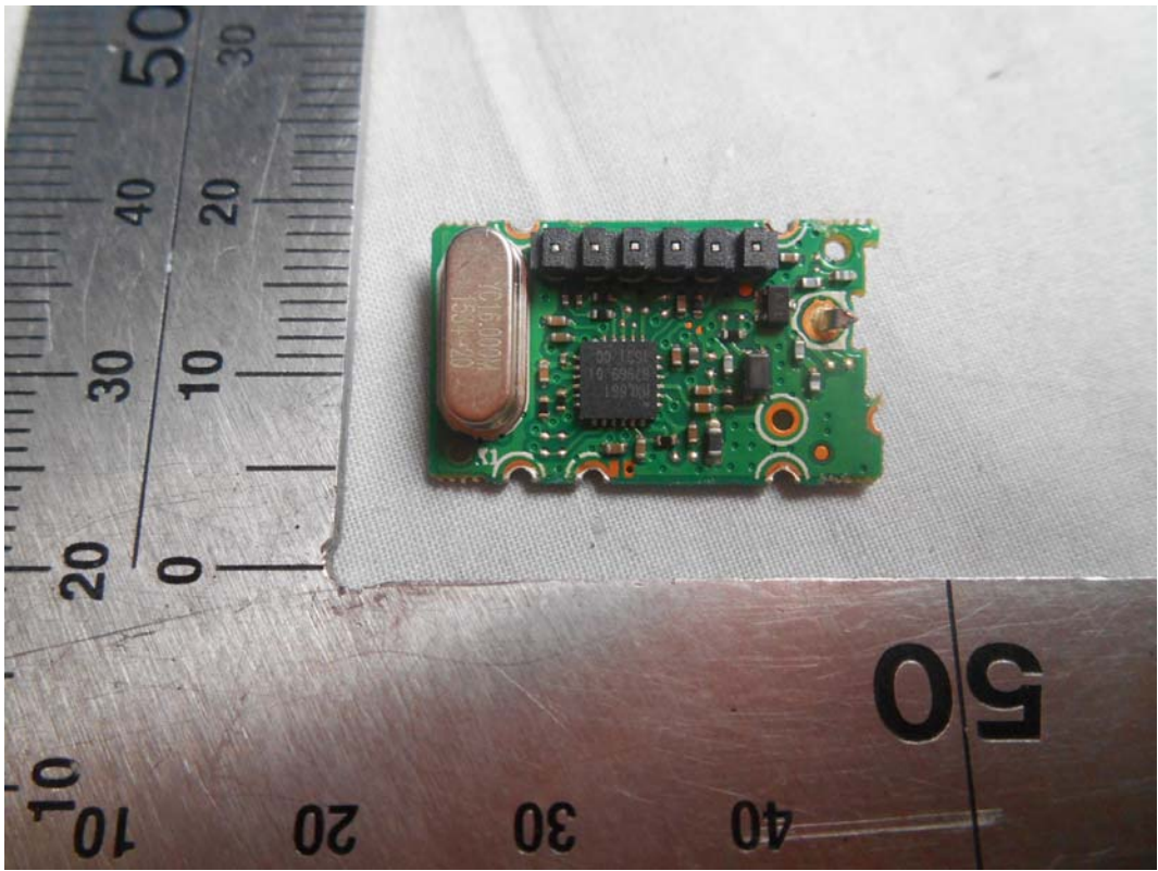
FIGURE 8 LED LCD TV (M/N: LTDN65K550GUWUS) TUNER BOARD (COMPONENT SIDE)
