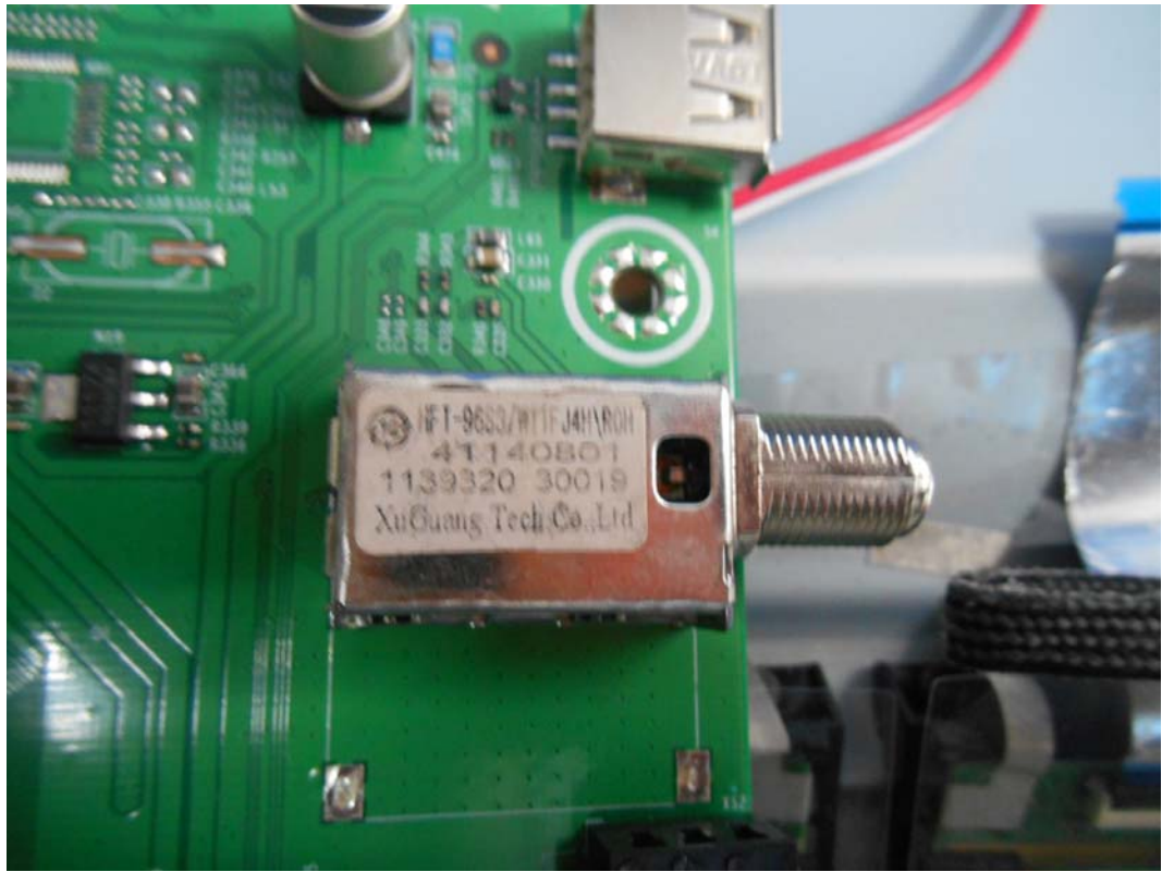
FIGURE 8 LED LCD TV (M/N: 50H6GB) TUNER ON MAIN BOARD
