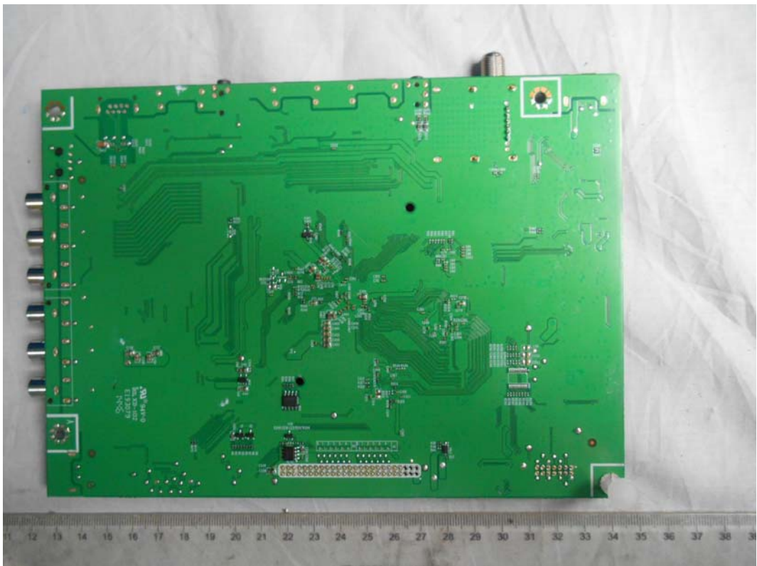
FIGURE 5 LED LCD TV (M/N: 50H6GB) MAIN BOARD (SOLDERED SIDE)
