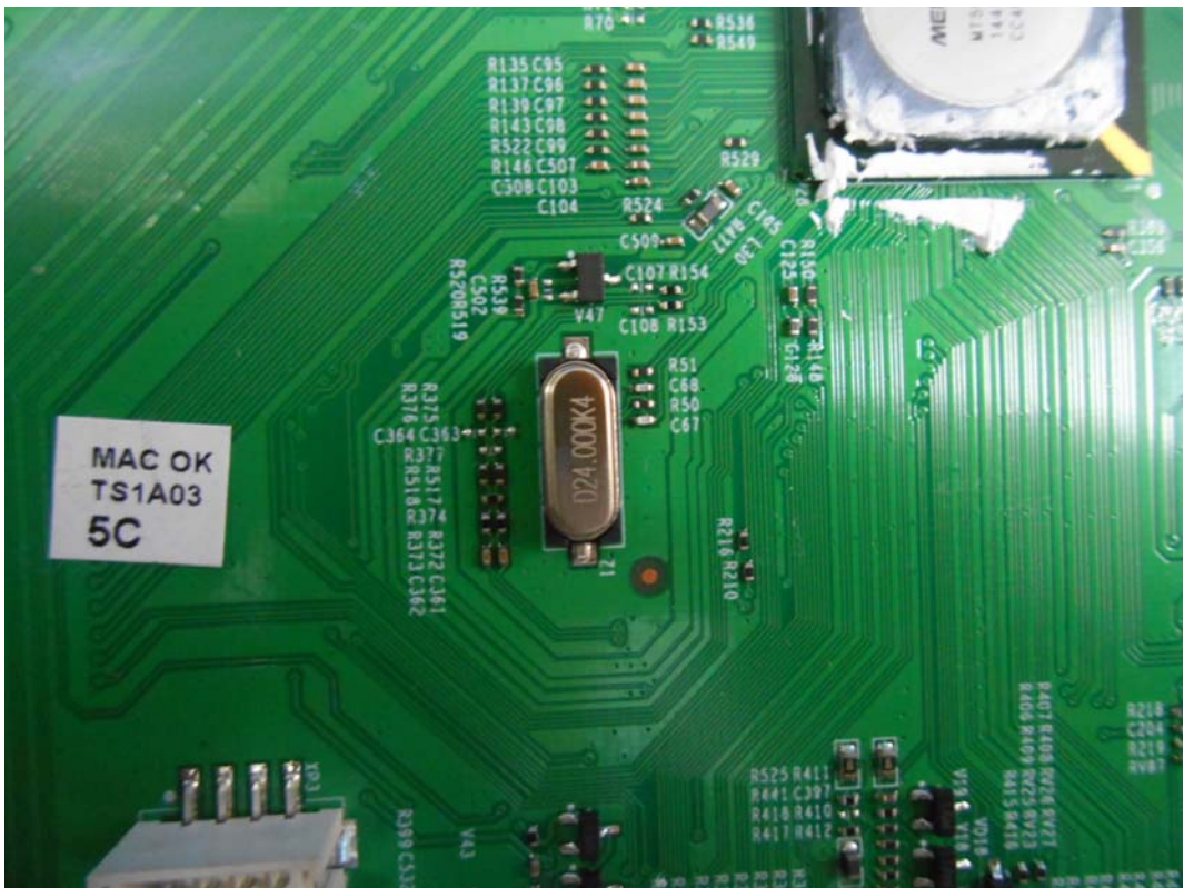
FIGURE 7 LED LCD TV (M/N: 50H6GB) CRYSTAL #2 ON MAIN BOARD
