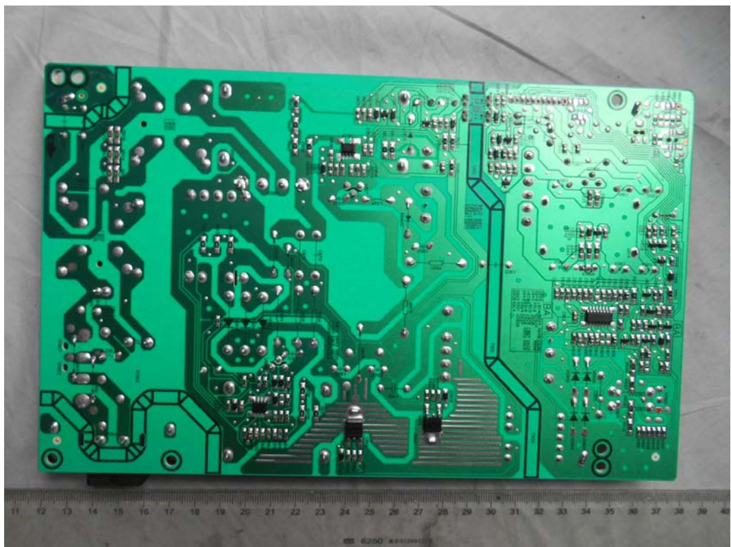
FIGURE 17 LED LCD TV (M/N: 50H6GB) POWER BOARD (SOLDERED SIDE)
