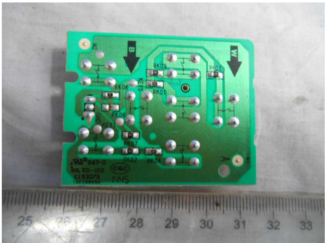
FIGURE 10 LED LCD TV (M/N: 50H6GB) KEY BOARD (SOLDERED SIDE)
