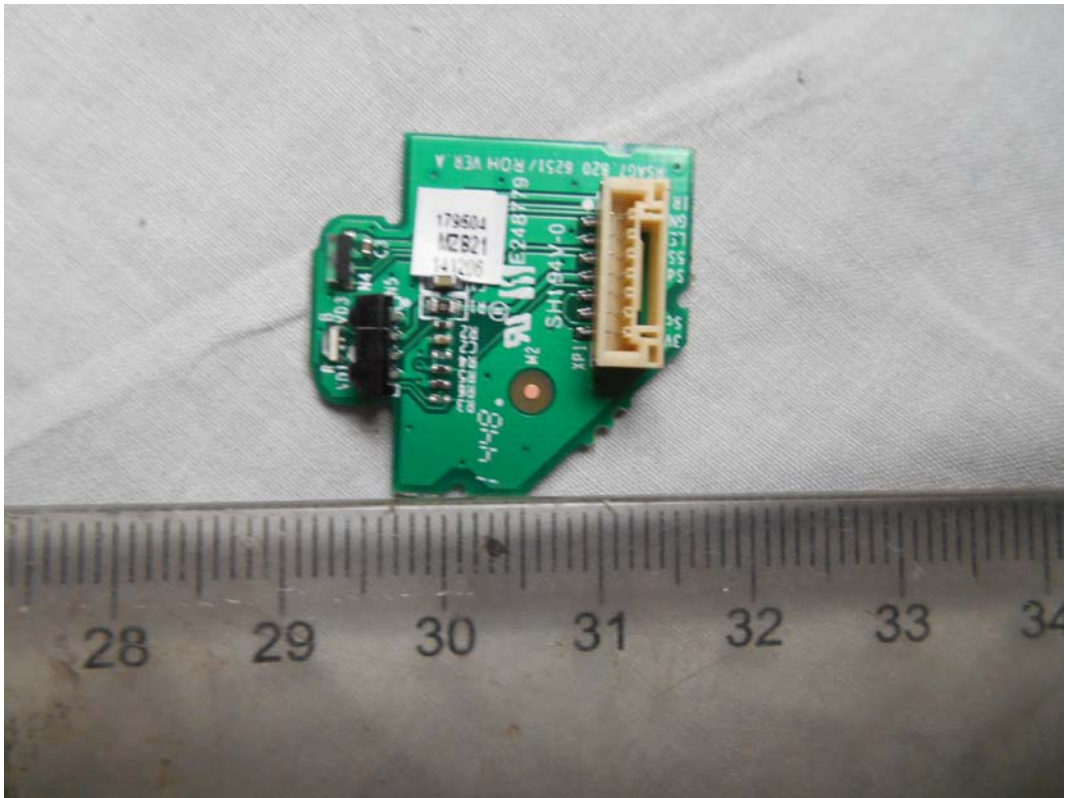
FIGURE 18 LED LCD TV (M/N: 50H6GB) INTERFACE BOARD (COMPONENT SIDE)
