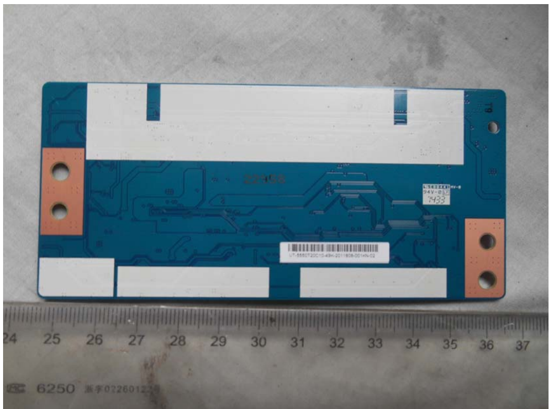
FIGURE 15 LED LCD TV (M/N: 50H6GB) SIGNAL BOARD (SOLDERED SIDE)
