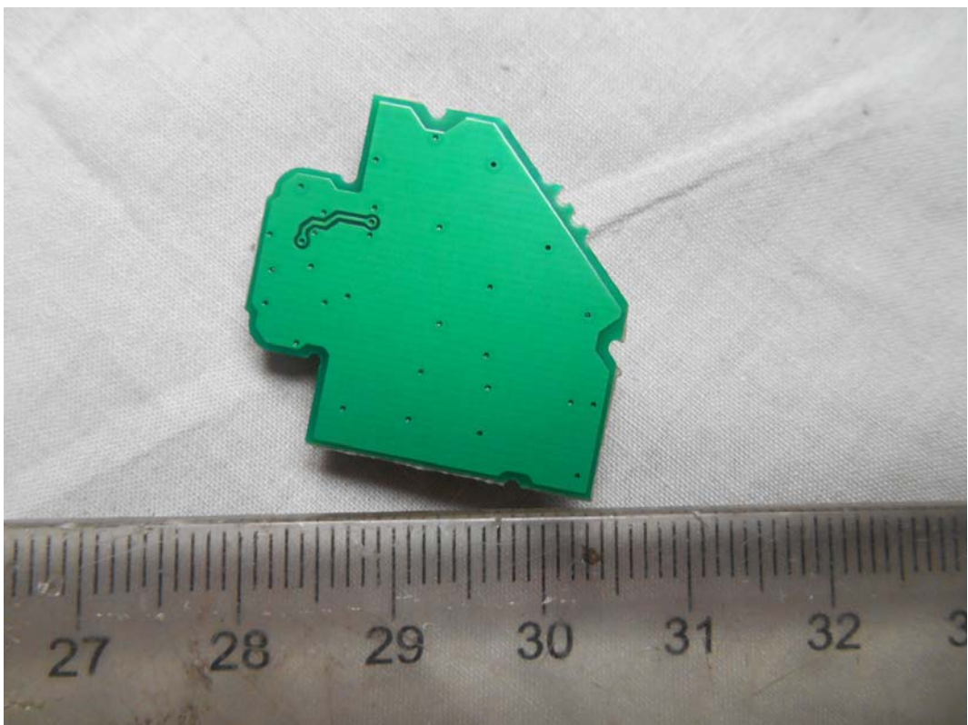
FIGURE 19 LED LCD TV (M/N: 50H6GB) INTERFACE BOARD (SOLDERED SIDE)
