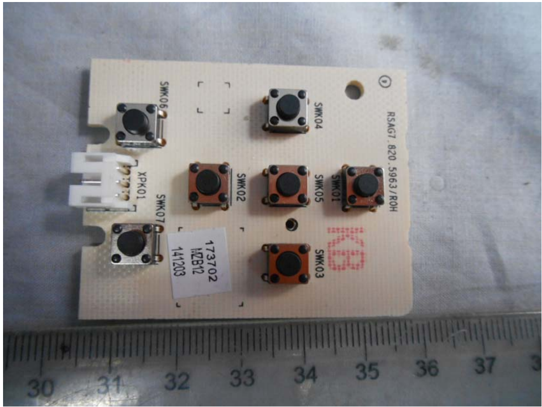
FIGURE 9 LED LCD TV (M/N: 50H6GB) KEY BOARD (COMPONENT SIDE)
