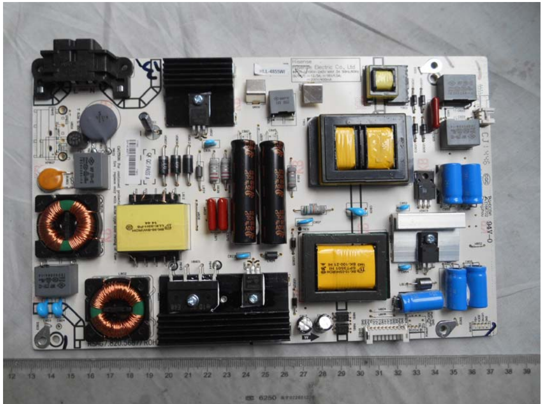
FIGURE 16 LED LCD TV (M/N: 50H6GB) POWER BOARD (COMPONENT SIDE)
