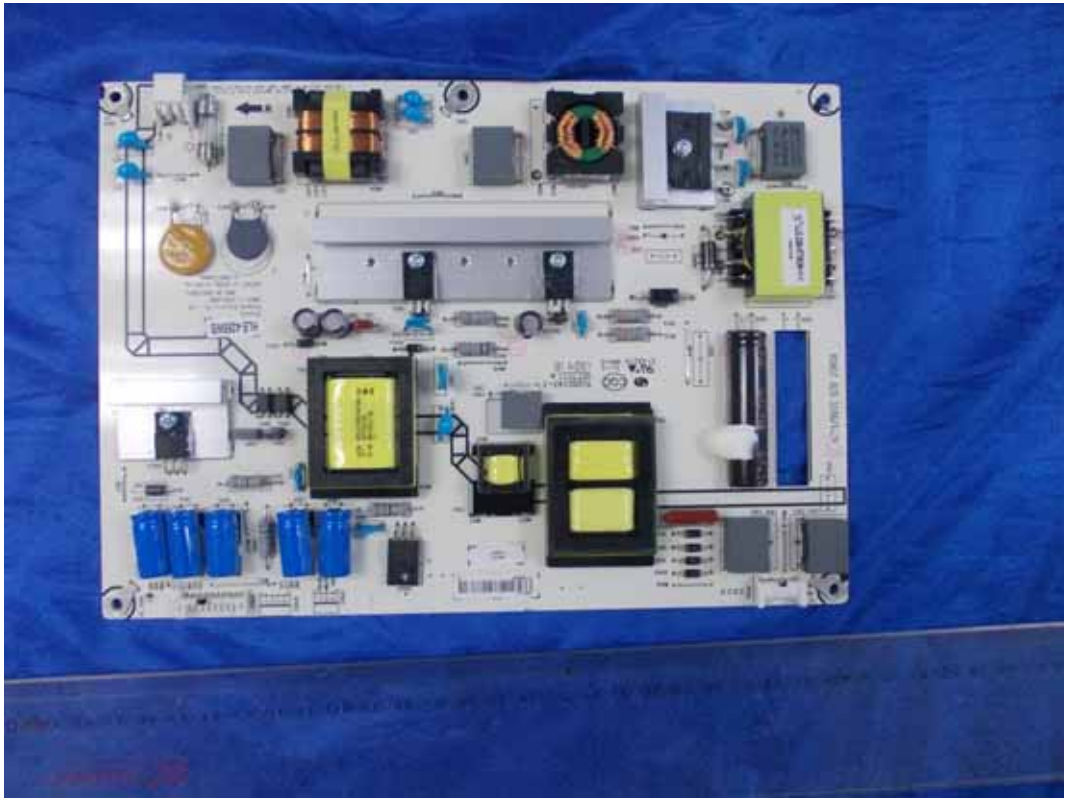
FIGURE 3 LED LCD TV (M/N: 55K362G) POWER BOARD (COMPONENT SIDE)
