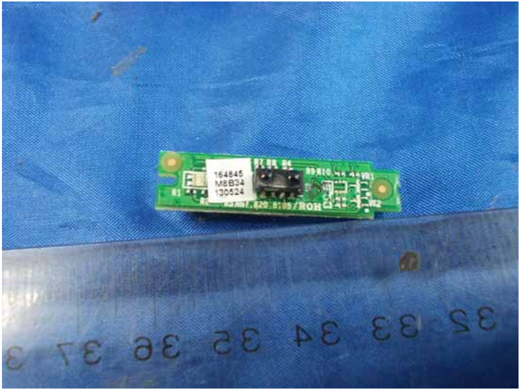
FIGURE 11 LED LCD TV (M/N: 55K362G) IR BOARD (COMPONENT SIDE)
