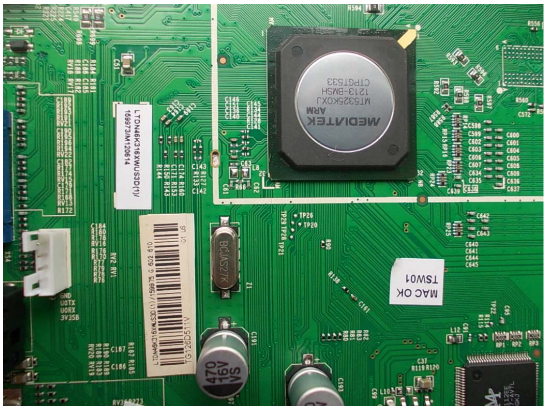
FIGURE 8 LED LCD TV(M/N: LTDN46K316XWUS3D) CHIP ON MAIN BOARD
