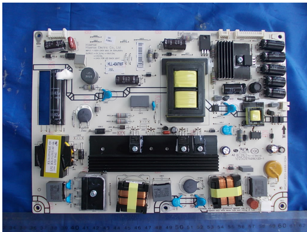
FIGURE 3 LED LCD TV (M/N: LTDN46K316XWUS3D) POWER BOARD (COMPONENT SIDE)
