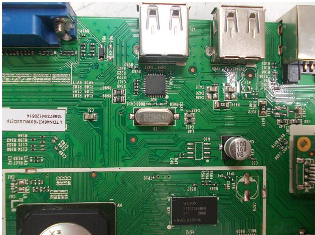
FIGURE 10 LED LCD TV(M/N: LTDN46K316XWUS3D) CRYSTAL #2 ON MAIN BOARD
