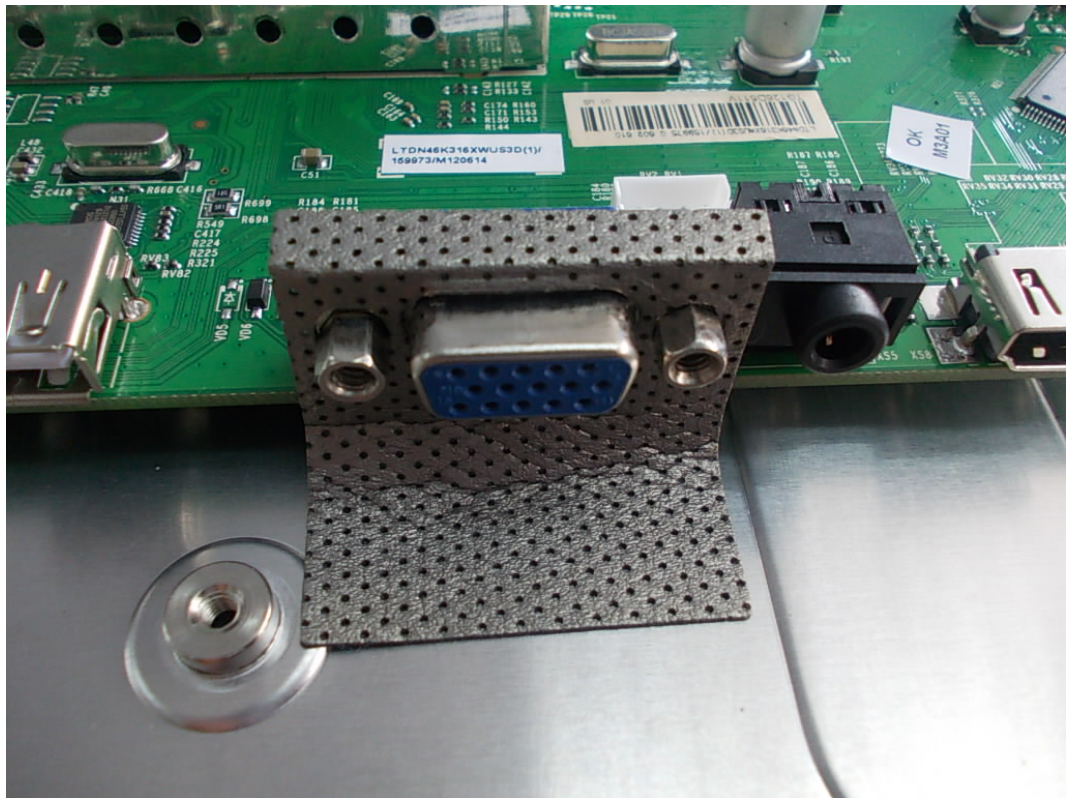
FIGURE 20 LED LCD TV (M/N: LTDN46K316XWUS3D) DEBUG #3
