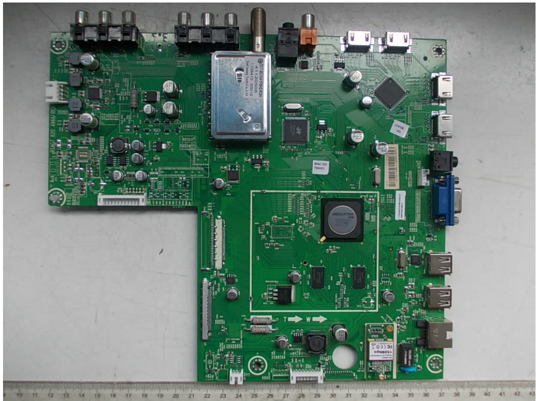
FIGURE 5 LED LCD TV (M/N: LTDN46K316XWUS3D) MAIN BOARD (COMPONENT SIDE)
