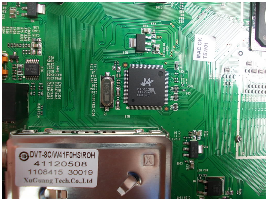
FIGURE 9 LED LCD TV(M/N: LTDN46K316XWUS3D) CHIP #1 & CRYSTAL #1 ON MAIN BOARD
