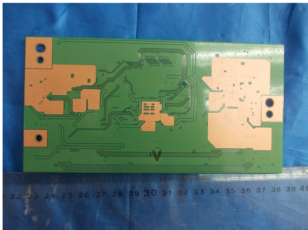
FIGURE 17 LED LCD TV (M/N: LTDN46K316XWUS3D) LCD PANEL CONTROL BOARD (SOLDERED SIDE)
