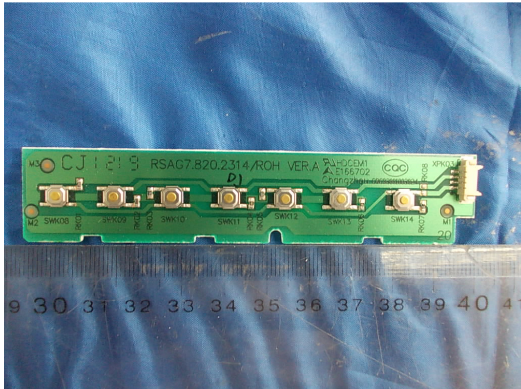
FIGURE 12 LED LCD TV (M/N: LTDN46K316XWUS3D) KEY BOARD (COMPONENT SIDE)
