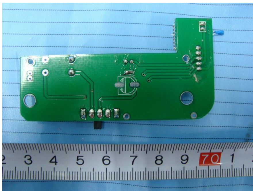
EUT – Power Button Board Bottom View
