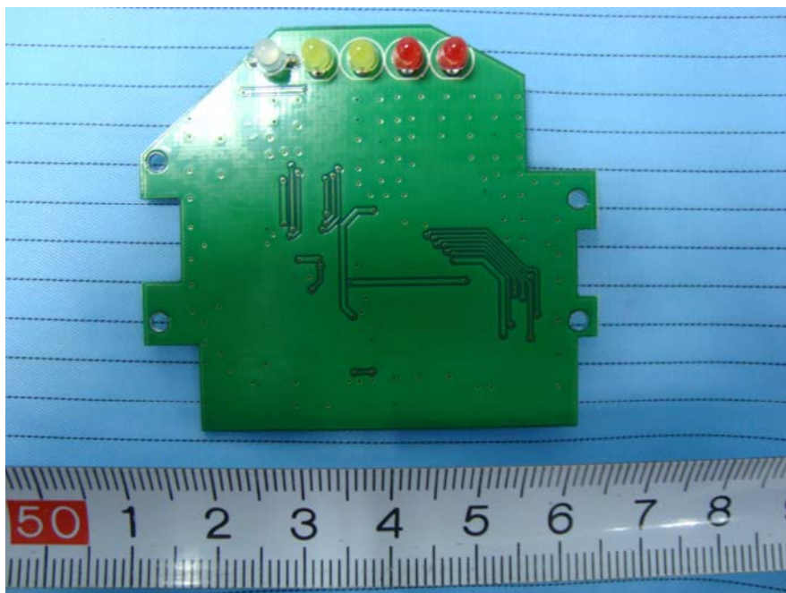
EUT – Display Control Board Bottom View
