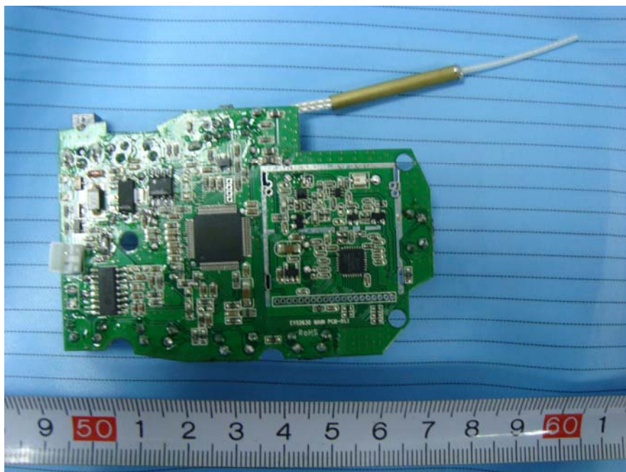
EUT – RF Board Unshielded Top View
