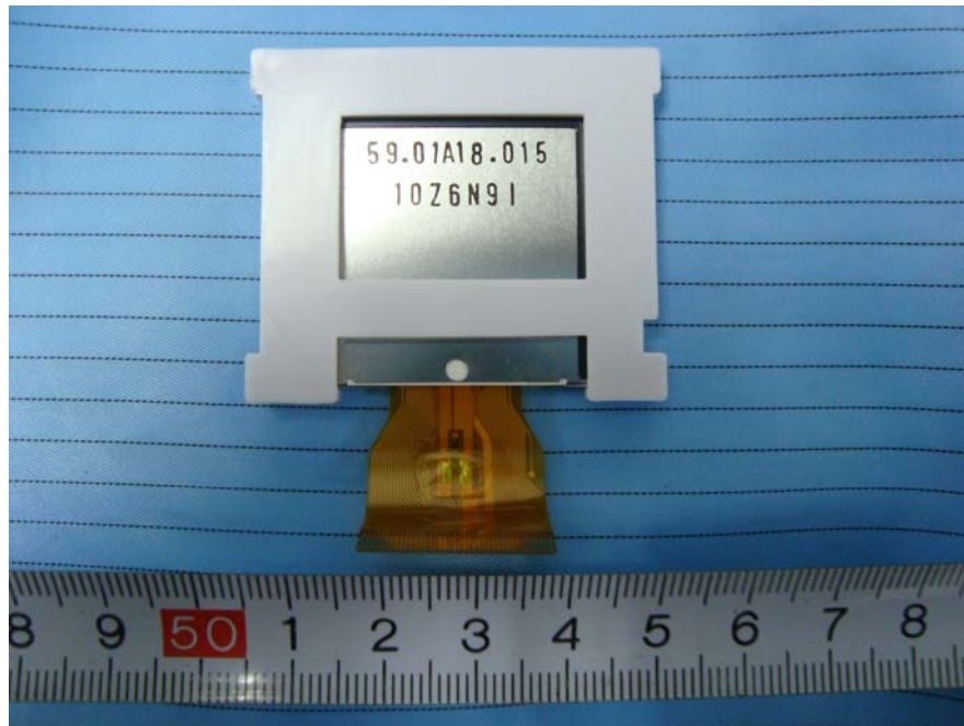
EUT – LCD Board (Display Temperature Function) Top View
