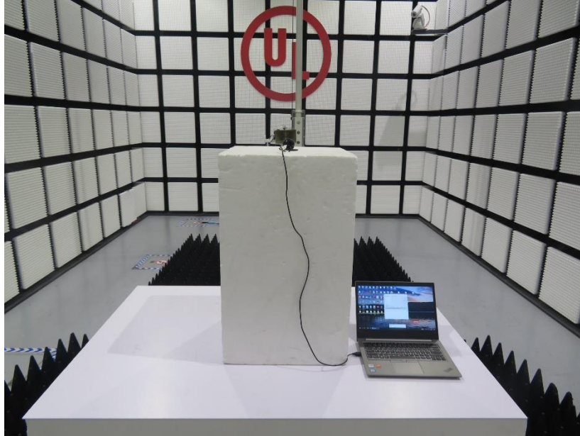
MEASUREMENT POSITION
