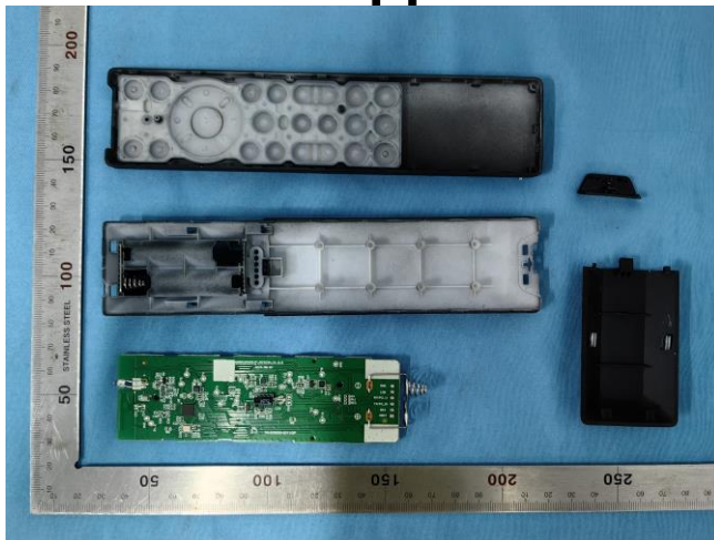
Internal Structure 1
