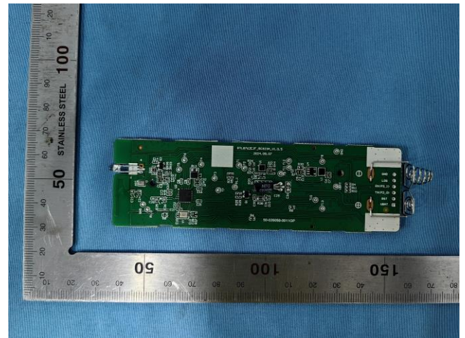
Internal Structure 2
