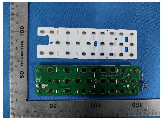
Internal Structure 4
