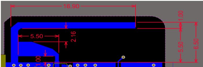
Unit: mm
