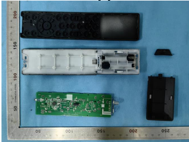
Internal Structure 1
