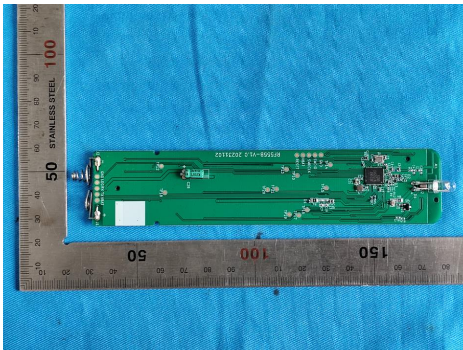
Mainboard Front
