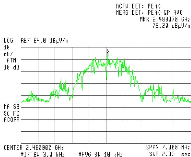
Figure 32 — 2480 MHz
