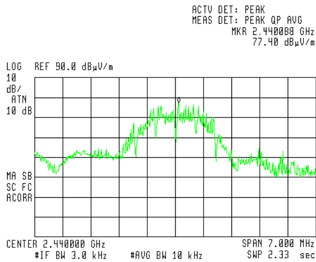
Figure 31 — 2440 MHz
