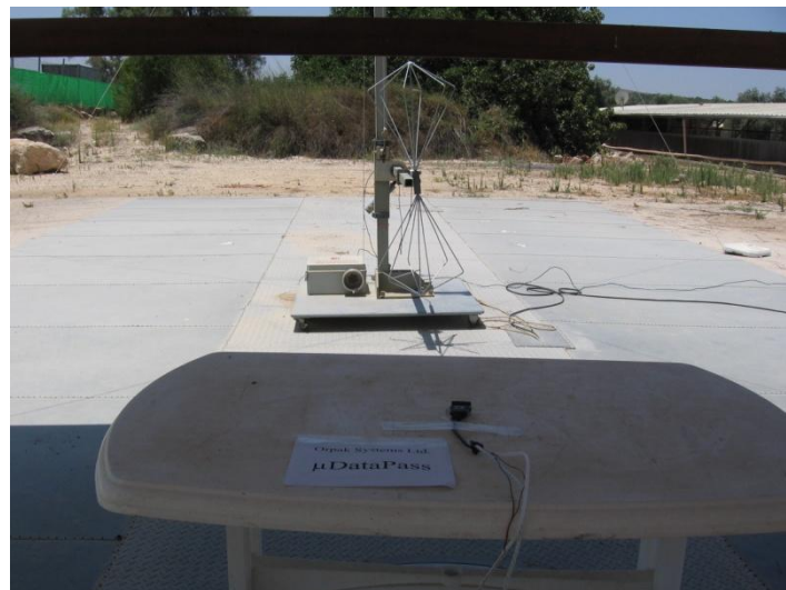
Figure 3. Radiated Emission Test Setup
