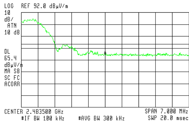
Figure 23 — 2480 MHz
