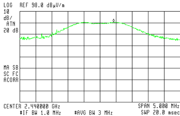
Figure 18 — 2440 MHz
