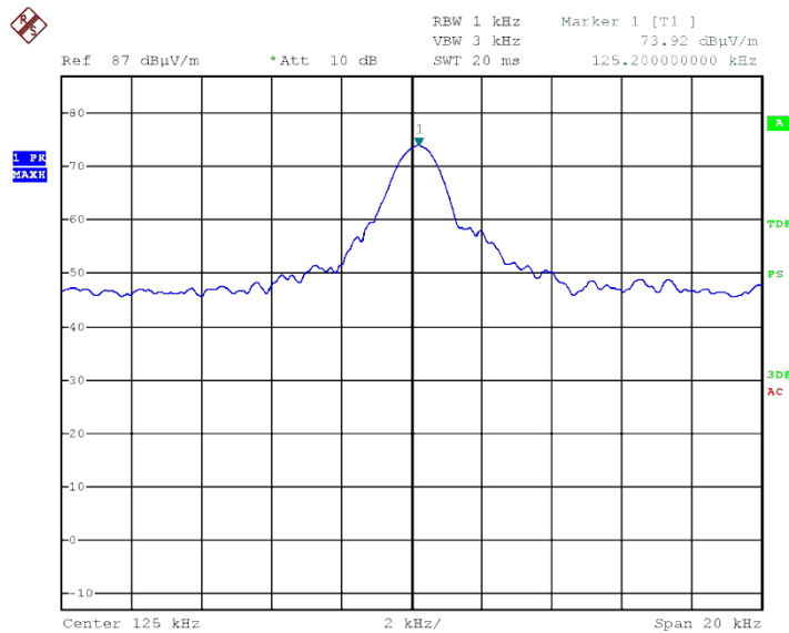
Figure 10. Field Strength of Fundamental, Vertical
