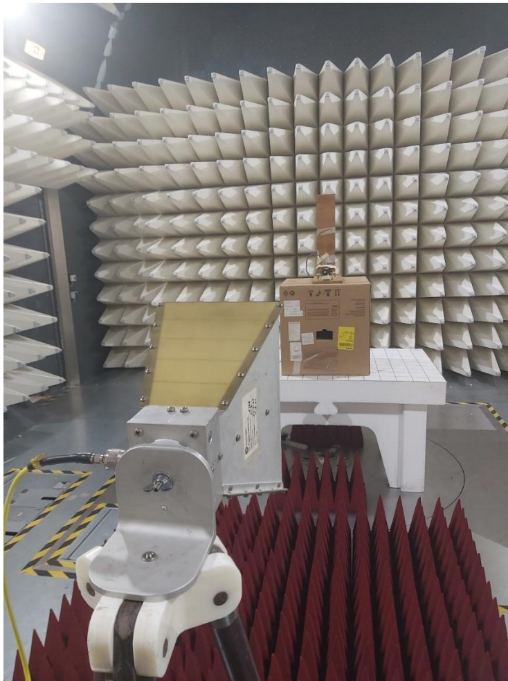
Figure 1 Radiated emission, 1.0-18.0 GHz
