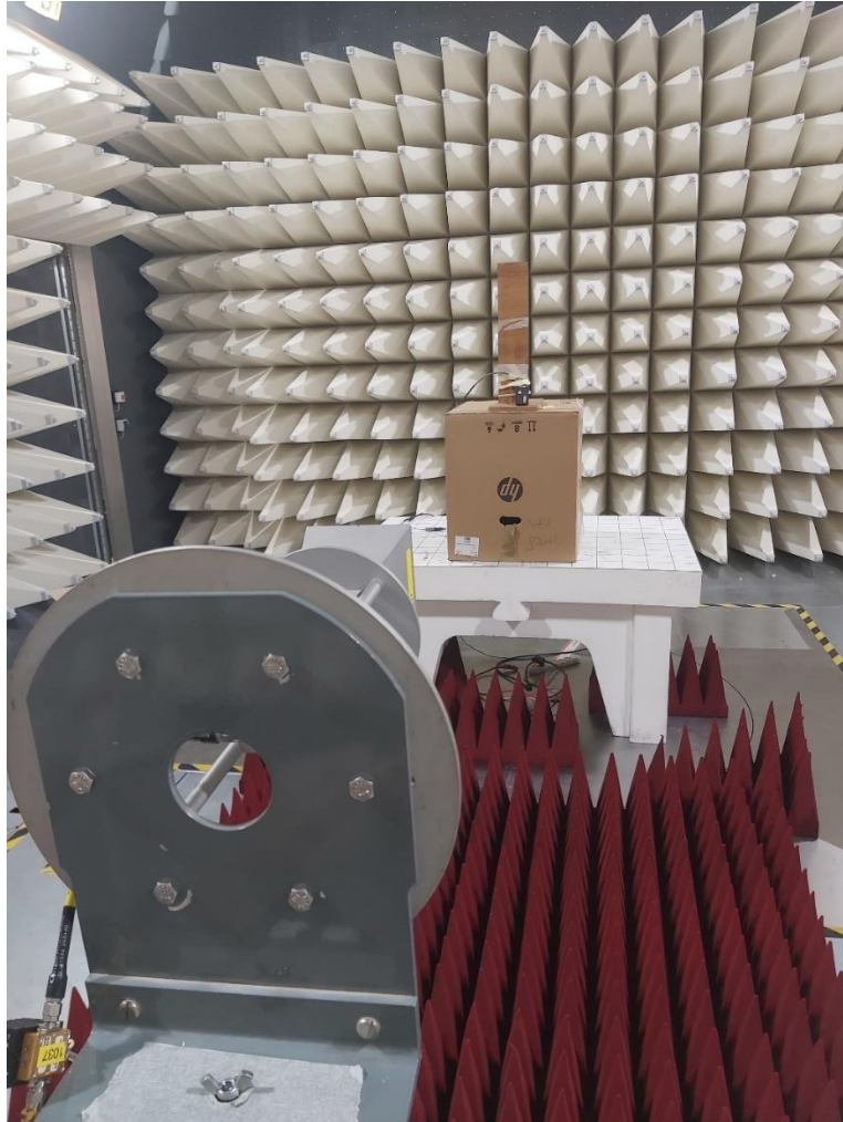
Figure 2 Radiated emission, 18-26.5 GHz
