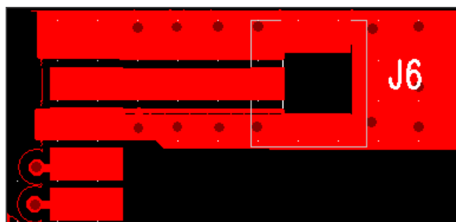
Figure 1. Top Layer
