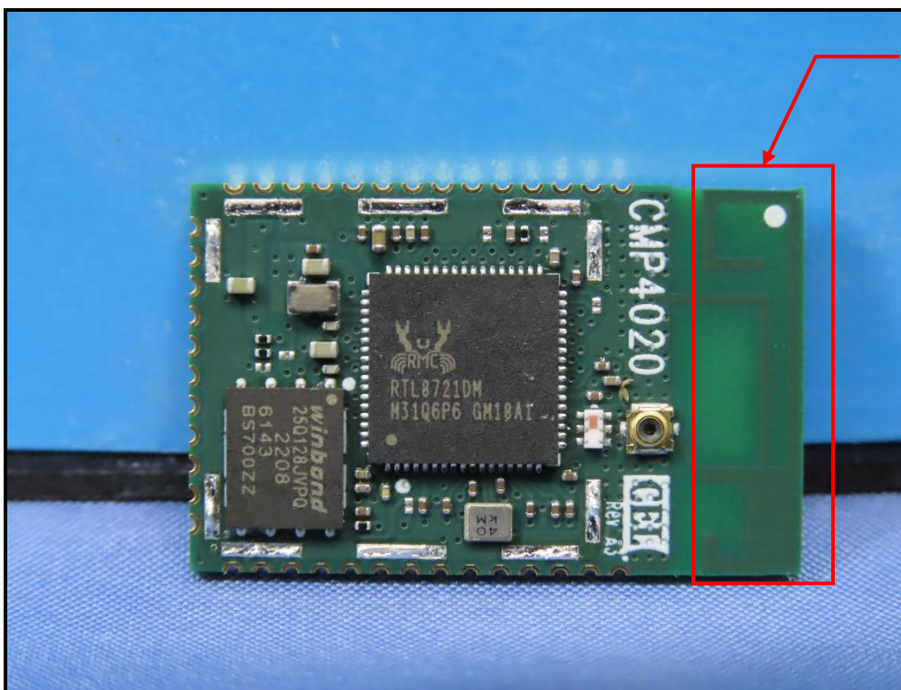
Antenna No.2
