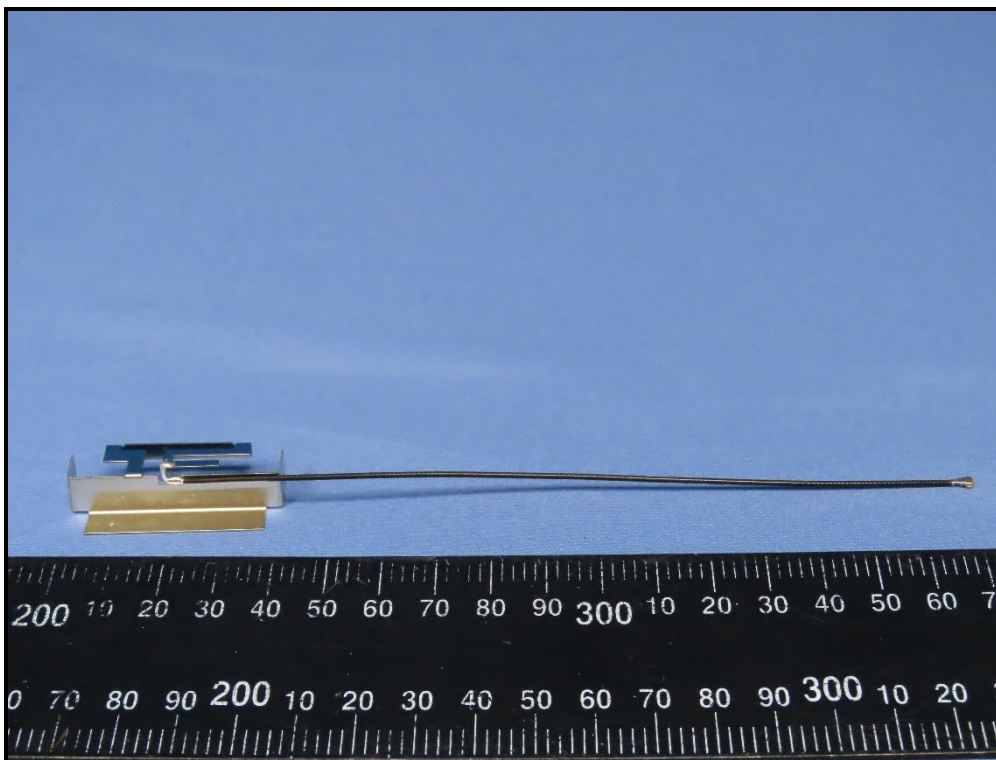
Antenna 1 (Brand: MAG.LAYERS, Model: MSA-4008-25GC1-A2)
